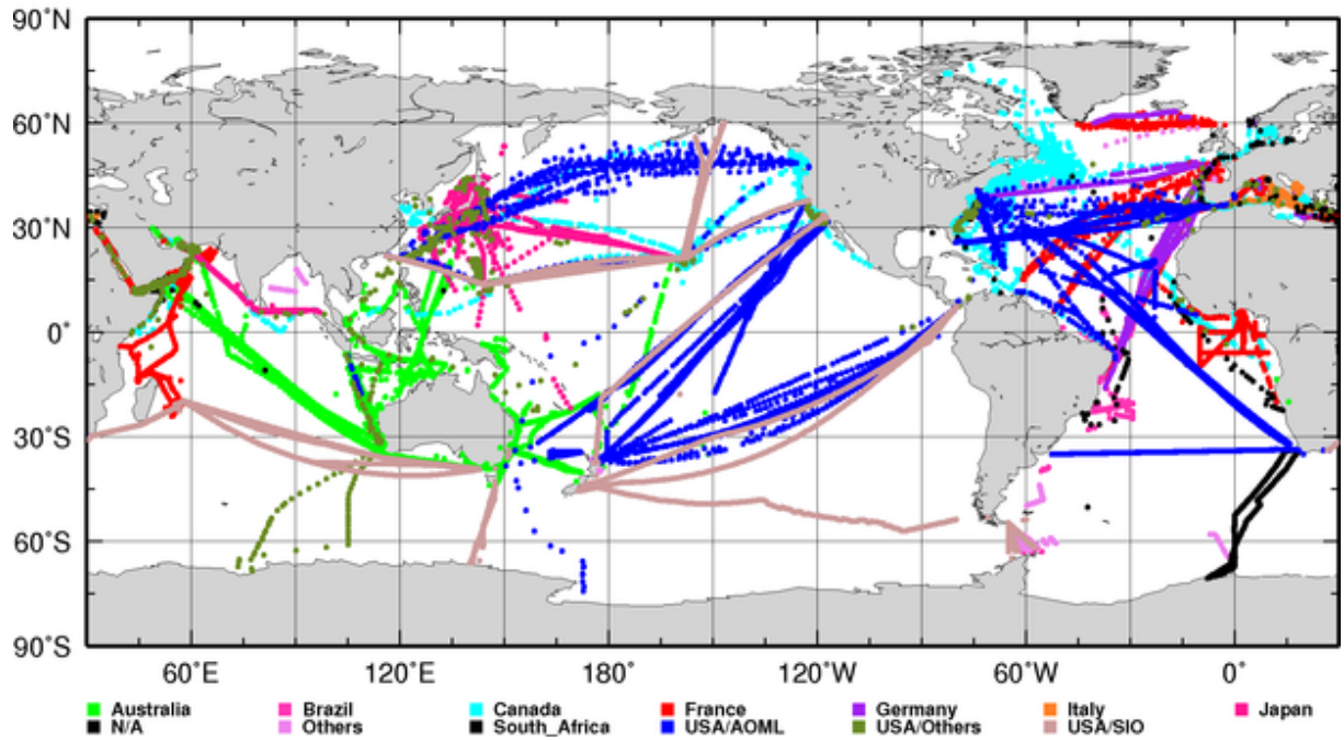
XBT Deployments Y2006 (Total 27998)
