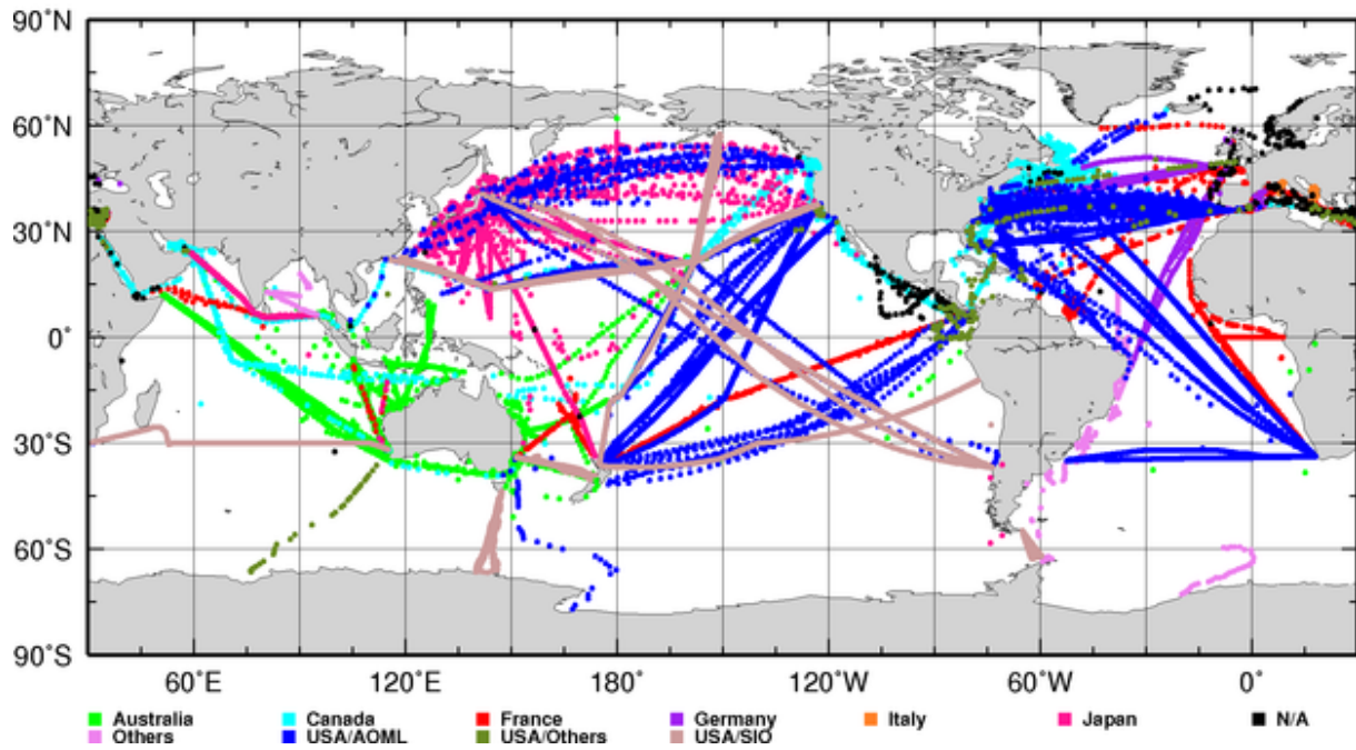
XBT Deployments Y2003 (Total 28744)
