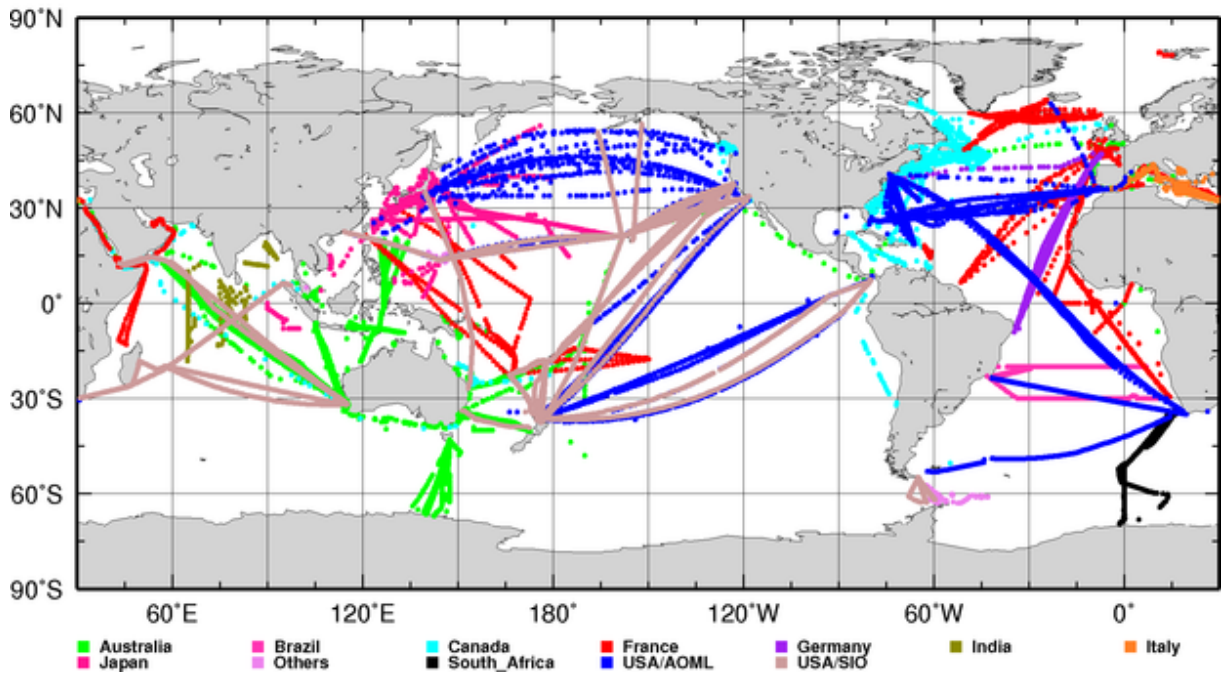
XBT Deployments Y2009 (Total 24173)
