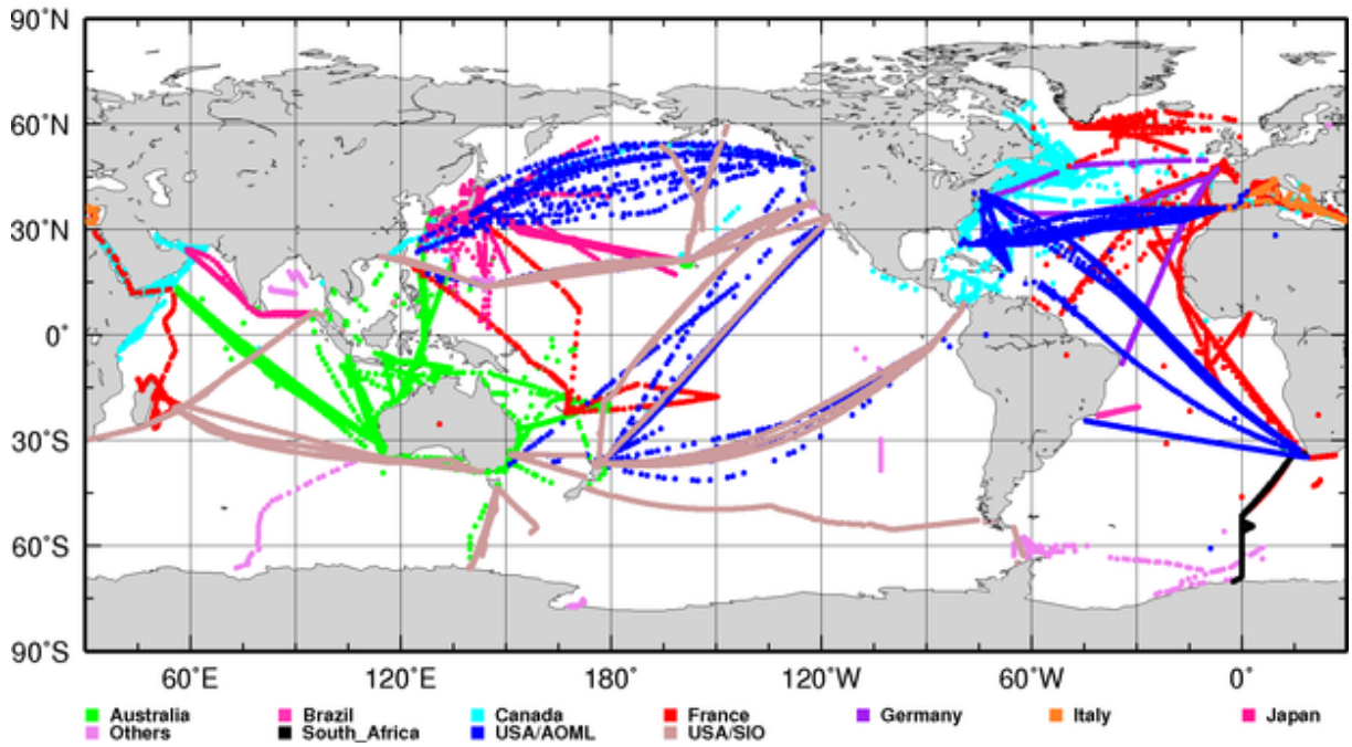
XBT Deployments Y2008 (Total 25231)
