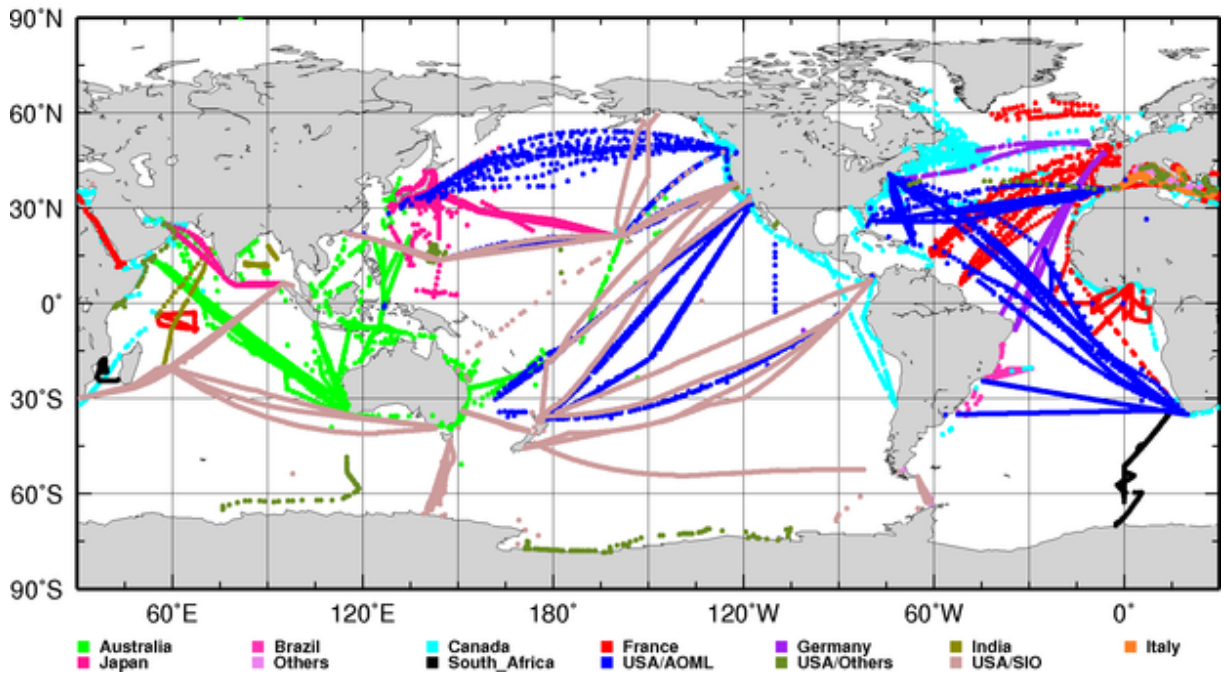
XBT Deployments Y2007 (Total 24115)
