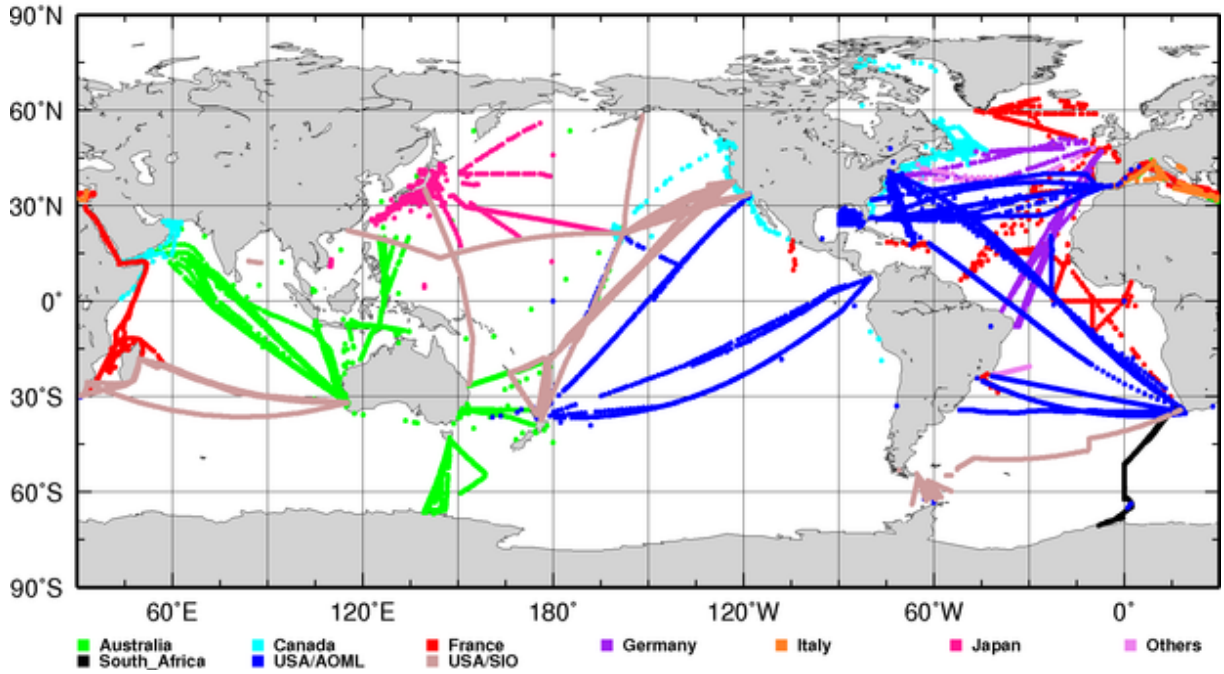
XBT Deployments Y2010 (Total 19150)
