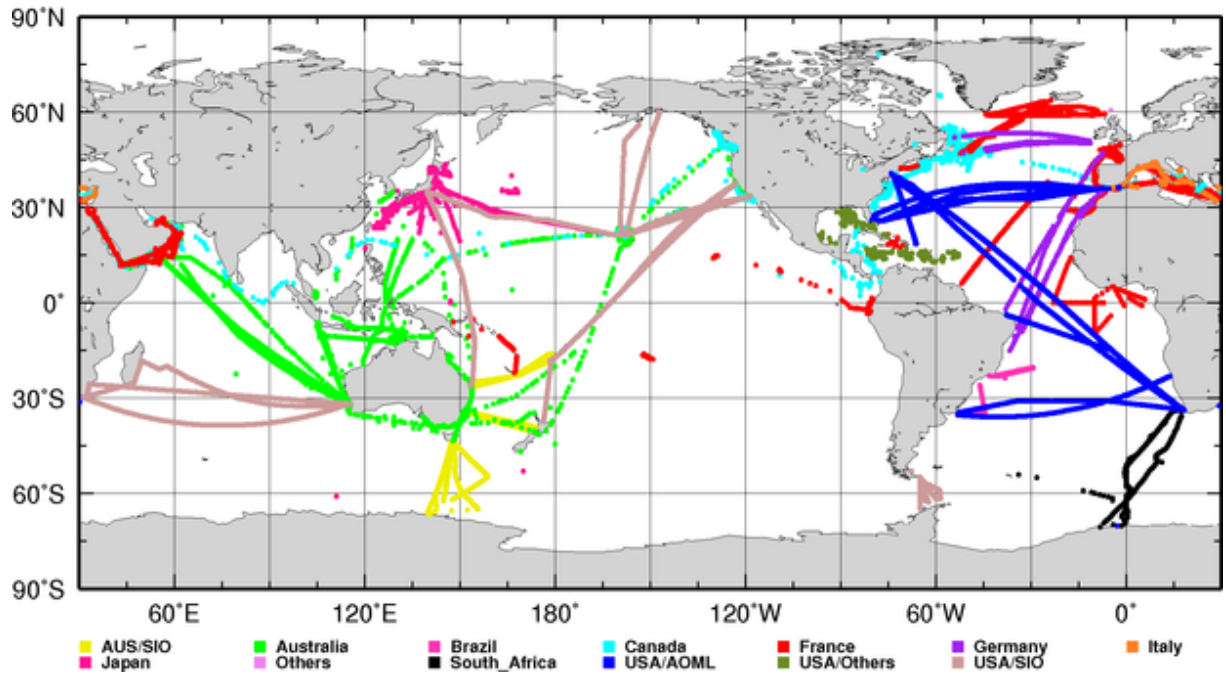
XBT Deployments Y2012 (Total 18581)
