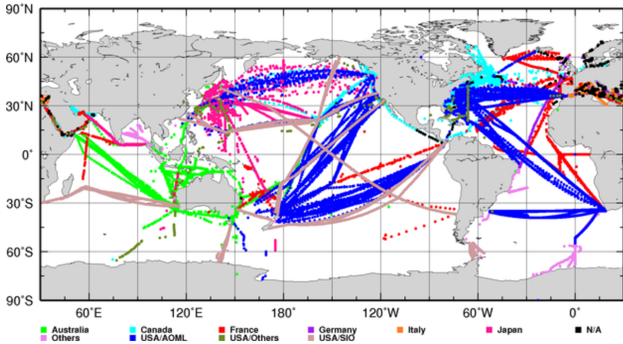
XBT Deployments Y2004 (Total 34553)
