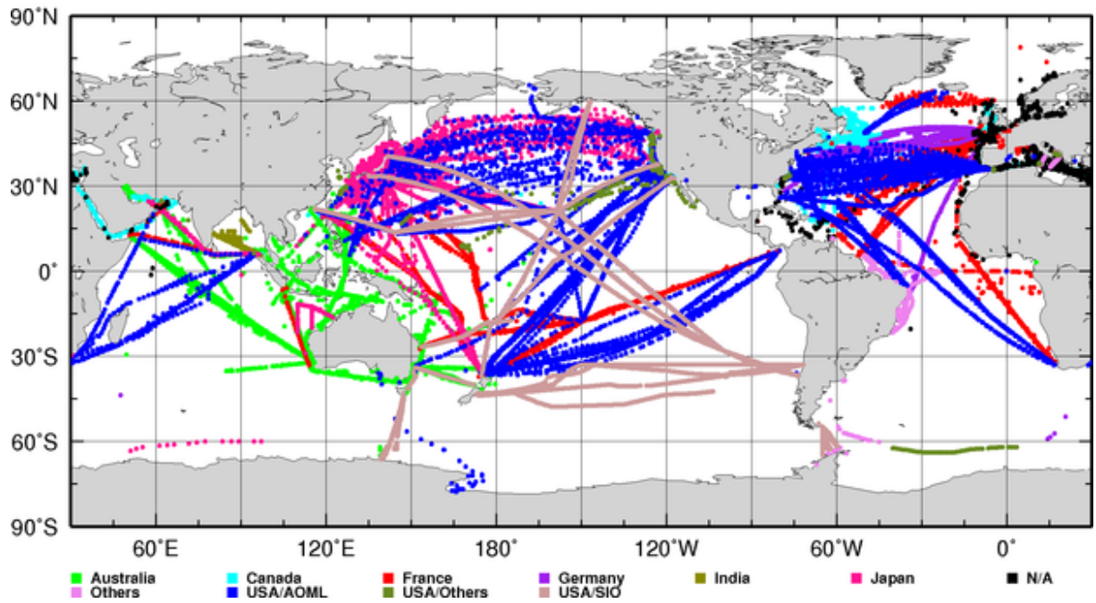
XBT Deployments Y2001 (Total 33845)
