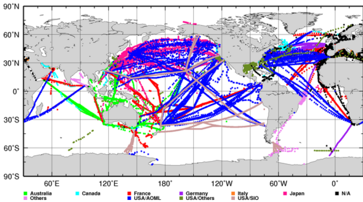
XBT Deployments Y2000 (Total 42138)
