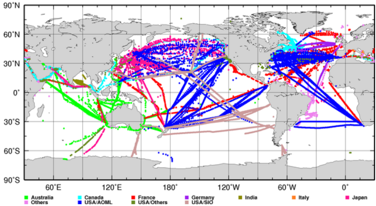
XBT Deployments Y2002 (Total 31386)
