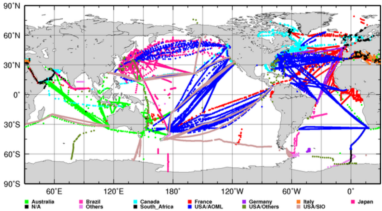
XBT Deployments Y2005 (Total 31567)
