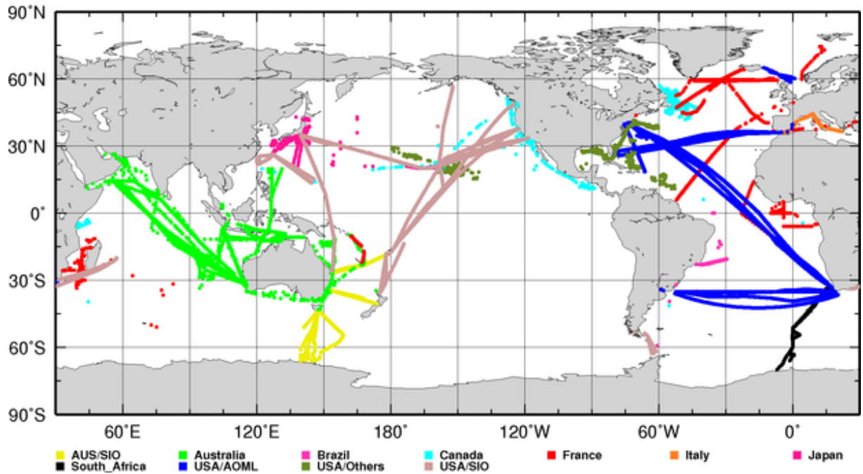
XBT Deployments Y2014 (Total 20040)
