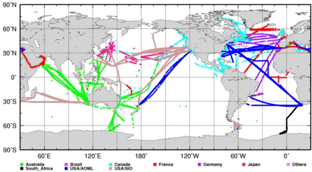
XBT Deployments Y2011 (Total 17610)
