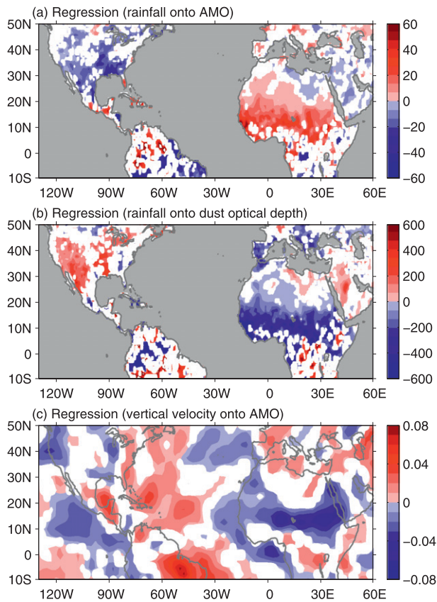
FIG. 6. Linkage of the AMO, rainfall, and aerosol. Shown are (a) regression ( \text{mm month}^{-1} \text{ }^{\circ}\text{C}^{-1} ) of annual rainfall anomalies onto the AMO index, (b) regression ( \text{mm month}^{-1} \text{ DAOD}^{-1} ) of annual rainfall anomalies onto the DAOD time series in the tropical North Atlantic, and (c) regression ( \text{Pa s}^{-1} \text{ }^{\circ}\text{C}^{-1} ) of annual 500-hPa vertical pressure velocity anomalies onto the AMO index. The regressions are calculated based on the 7-yr running mean data. Only regression coefficients exceeding the 95% significant level are plotted.
