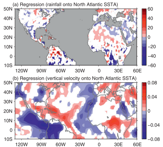
FIG. 7. Linkage of the North Atlantic SST with rainfall using the data with the linear trends included. Shown are (a) regression ( \text{mm month}^{-1} \text{ }^{\circ}\text{C}^{-1} ) of annual rainfall anomalies onto the North Atlantic SST index and (b) regression ( \text{Pa s}^{-1} \text{ }^{\circ}\text{C}^{-1} ) of annual 500-hPa vertical pressure velocity anomalies onto the North Atlantic SST index. The regressions are calculated based on the 7-yr running mean data. Only regression coefficients exceeding the 95% significant level are plotted.
