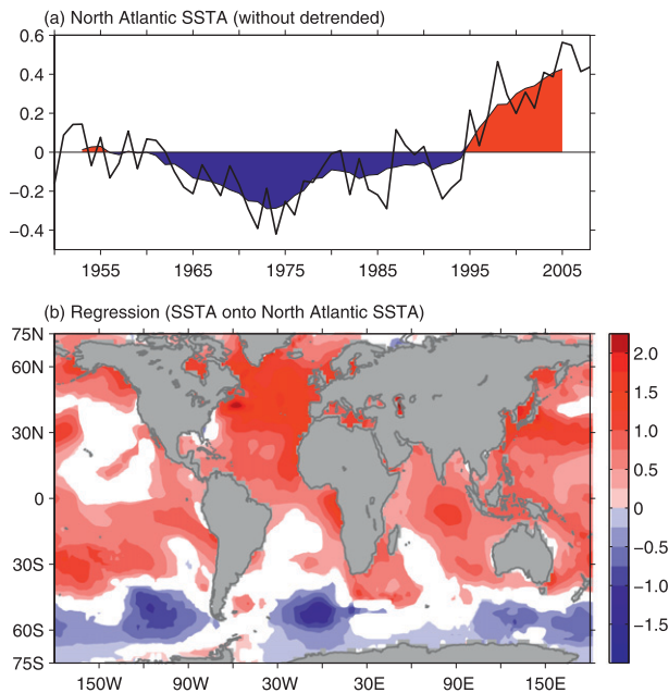
FIG. 4. The time series of the North Atlantic SST anomalies and its regressed map using the data with the linear trends included. Shown are (a) the annual SST anomalies ( ^{\circ}\text{C} ) in the North Atlantic of 0^{\circ} – 60^{\circ}\text{N} and from the east coast of the Americas to 0^{\circ} longitude and (b) regression ( ^{\circ}\text{C } ^{\circ}\text{C}^{-1} ) of global annual SST anomalies onto the North Atlantic SST index of (a). The regression is calculated based on the 7-yr running mean data. Only regression coefficients exceeding the 95% significant level are plotted. The shading in (a) represents the time series of 7-yr running means.
