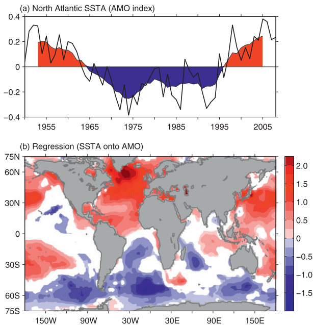
FIG. 1. The AMO index and its relationship with global ocean SST. Shown are (a) the detrended annual SST anomalies ( ^{\circ}\text{C} ) in the North Atlantic of 0^{\circ} – 60^{\circ}\text{N} and from the east coast of the Americas to 0^{\circ} longitude and (b) regression ( ^{\circ}\text{C } ^{\circ}\text{C}^{-1} ) of global annual SST anomalies onto the AMO index of (a). The regression is calculated based on the 7-yr running mean data. The shading in (a) represents the 7-yr running mean time series. Only regression coefficients exceeding the 95% significant level are plotted in (b).
