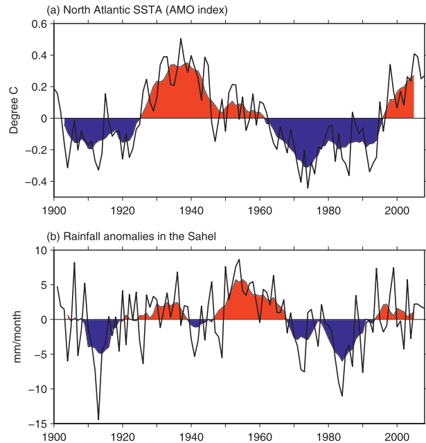
FIG. 3. The AMO index and Sahel rainfall time series for a long-term record of 1900–2008. Shown are (a) the AMO index ( ^{\circ}\text{C} ) and (b) the annual rainfall anomalies ( \text{mm month}^{-1} ) in the Sahel ( 10^{\circ}\text{--}20^{\circ}\text{N} , 20^{\circ}\text{W--}40^{\circ}\text{E} ). The time series are detrended and the shading represents the time series of 7-yr running means.
