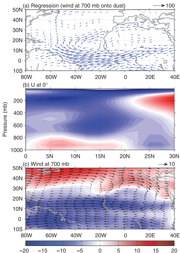
FIG. 11. Wind variations with dust and the mean winds. Shown are (a) regression ( \text{m s}^{-1} \text{DAOD}^{-1} ) of annual wind anomalies at 700 hPa onto the DAOD time series, (b) vertical–latitude section of the mean zonal wind at 0^\circ longitude during July–September, and (c) the mean winds (vector) and the mean zonal winds (shading) at 700 hPa during July–September. Winds are in \text{m s}^{-1} . The regression is calculated based on the detrended and 7-yr running mean data. Only regressions exceeding the 95% significant level are plotted.
