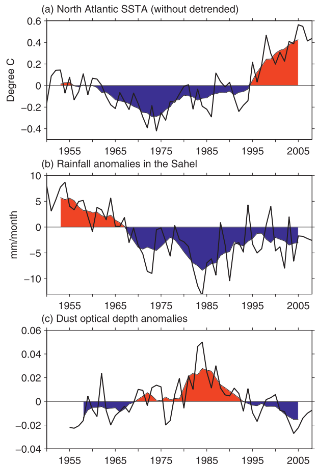
FIG. 5. The time series of the North Atlantic SST, Sahel rainfall, and dust in the tropical North Atlantic using the data with the linear trends included. Shown are (a) the annual SST anomalies ( ^{\circ}\text{C} ) in the North Atlantic of 0^{\circ} – 60^{\circ}\text{N} and from the east coast of the Americas to 0^{\circ} longitude, (b) the annual rainfall anomalies ( \text{mm month}^{-1} ) in the Sahel ( 10^{\circ} – 20^{\circ}\text{N} , 20^{\circ}\text{W} – 40^{\circ}\text{E} ), and (c) the annual DAOD anomalies in the tropical North Atlantic ( 0^{\circ} – 30^{\circ}\text{N} , 10^{\circ} – 65^{\circ}\text{W} ). The shading represents the time series of 7-yr running means.
