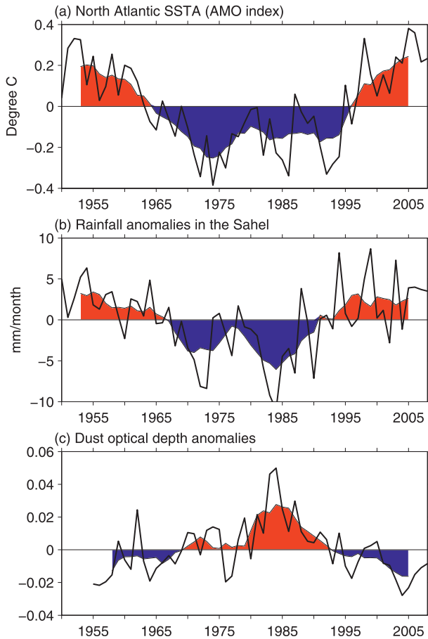
FIG. 2. The AMO, Sahel rainfall, and dust in the tropical North Atlantic. Shown are (a) the AMO index ( ^{\circ}\text{C} ), (b) the annual rainfall anomalies ( \text{mm month}^{-1} ) in the Sahel ( 10^{\circ}\text{--}20^{\circ}\text{N} , 20^{\circ}\text{W--}40^{\circ}\text{E} ), and (c) the annual DAOD anomalies in the tropical North Atlantic ( 0^{\circ}\text{--}30^{\circ}\text{N} , 10^{\circ}\text{--}65^{\circ}\text{W} ). The shading represents the time series of 7-yr running means.
