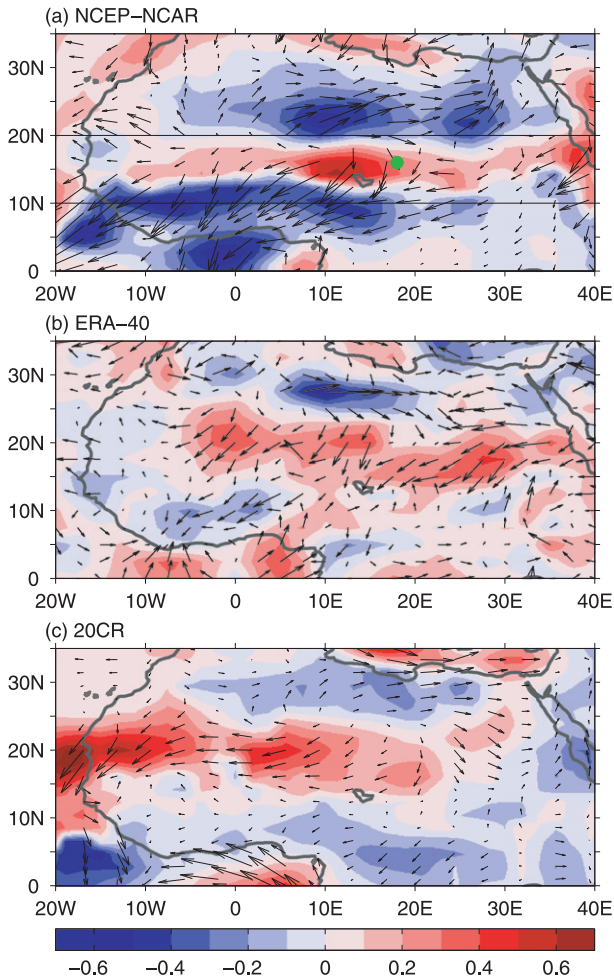
FIG. 9. Composite surface wind differences between the high and low dust years. Shown are from (a) the NCEP–NCAR reanalysis, (b) the ERA-40 reanalysis, and (c) the 20CR reanalysis. The shading represents the wind speed ( \text{m s}^{-1} ). The top and bottom quartiles of the DAOD time series are identified as the high and low dust years, respectively. For the NCEP–NCAR and 20CR, the 13 high dust years are 1962, 1973, 1974, 1975, 1979, 1981, 1983, 1984, 1985, 1986, 1987, 1988, and 1991; the 13 low dust years are 1955, 1956, 1957, 1958, 1961, 1964, 1976, 1977, 1996, 2003, 2004, 2005, and 2006. For the ERA-40, the 11 high dust years are 1962, 1973, 1974, 1975, 1979, 1981, 1983, 1984, 1985, 1986, and 1987; the 11 low dust years are 1958, 1961, 1964, 1965, 1968, 1976, 1977, 1993, 1995, 1996, and 2001. The green dot in (a) represents the Bodélé Depression in northern Chad—an area of some 40 000 \text{km}^2 centered on 16°N and 18°E (Washington and Todd 2005).
