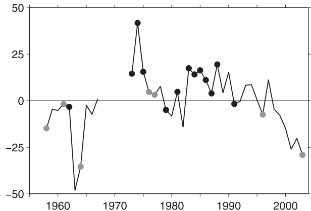
FIG. 10. Time series of the annual average of the wind speed cube ( \text{m}^3 \text{ s}^{-3} ) from the observed station data of Mahowald et al. (2007) in the western Sahel (13°–22°N, 20°W–15°E). The time series is linearly detrended. The black (gray) dots represent high (low) dust years used in the calculation of Fig. 9.
