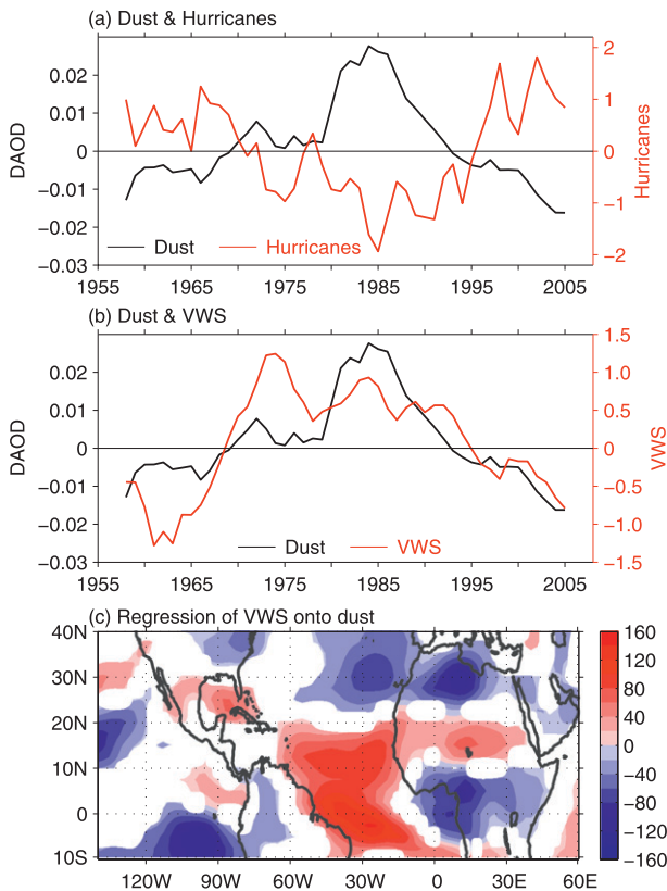
FIG. 8. Relationships of dust with Atlantic hurricanes and VWS. Shown are (a) the time series of DAOD and the number of Atlantic hurricanes, (b) the time series of DAOD and VWS, and (c) regression ( \text{m s}^{-1} \text{DAOD}^{-1} ) of VWS onto the DAOD time series in the tropical North Atlantic. In (b), the VWS is calculated as the magnitude of the vector difference between winds at 200- and 850-hPa in the main development region of 10^{\circ} – 20^{\circ} N, 85^{\circ} – 15^{\circ} W during the hurricane season of June–November. The correlations of dust with the number of hurricanes and VWS at 0 lag are -0.79 and 0.69 , respectively. The regression is calculated based on the 7-yr running mean data. Only regression coefficients exceeding the 95% significant level are plotted.
