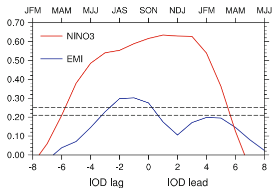
Fig. 1 Lead-lag correlations of the IOD index with El Niño Modoki index (EMI) and NINO3 index during 1950–2008. The IOD index during Sept–Oct–Nov (SON) is represented by month 0 or zero lag. The dashed lines indicate 95 and 99 % significant levels, respectively
