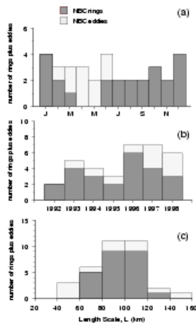
Figure 4: (a) Months in which rings and eddies are formed, (b) number of rings and eddies observed during each year, and (c) length scale (in km) of the rings and eddies.
