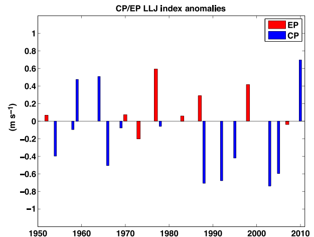
Figure 6. Values of the GPLLJ index (see text for its definition) calculated for the 21 major El Niño events after 1950. The blue bars indicate CP El Niño events, and the red bars indicate EP El Niño events.
