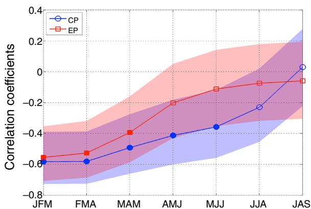
Figure 5. Correlation coefficients between the CP and EP ENSO indices and the SLP anomalies averaged in a region between 20^{\circ} – 25^{\circ} N and 80^{\circ} – 90^{\circ} W [i.e. the dashed square boxes in Figure 2 (a) and (b)]. Filled symbols indicate statistically significant points with p -value less than 0.05. The shaded area indicates 95% confidence interval for coefficients.
