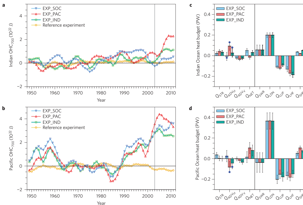
Figure 4 | \text{OHC}_{700} and heat budget for three sensitivity experiments. a, b , Time series of \text{OHC}_{700} for the Indian ( a ) and Pacific ( b ) oceans derived from EXP_SOC, EXP_PAC, EXP_IND, and the reference experiment. c, d , Heat budget terms for the Indian ( c ) and Pacific ( d ) oceans derived from EXP_SOC, EXP_PAC, and EXP_IND relative to the reference experiment are averaged for 2003–2012. The error bars show the 90% confidence levels derived from the six-member ensemble runs. The blue circles in c, d indicate the values for inter-ocean heat transport via the Indonesian passages. EXP_SOC, EXP_PAC and EXP_IND are identical to the control experiment except that real-time winds were applied only over the Southern, Pacific and Indian oceans, respectively. Inter-ocean heat transport increased in both EXP_PAC and EXP_IND but was almost unchanged in EXP_SOC.
