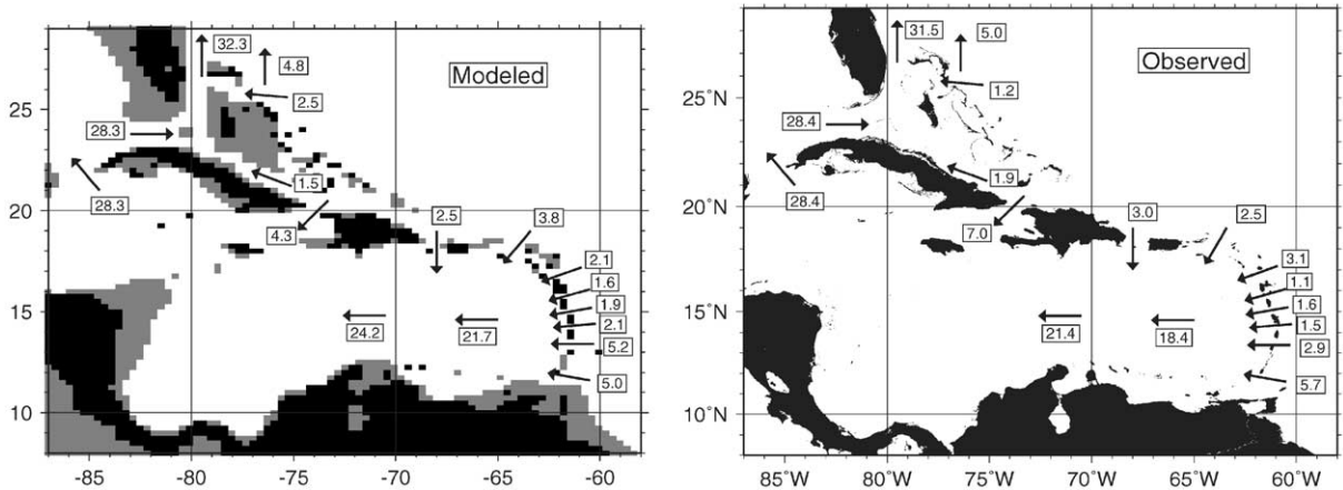
Fig. 14. Comparison of Caribbean passage transports from the combined wind/MOC-forced model simulation with observed passage transports, as summarized in Table 2.
