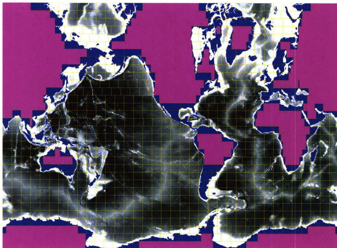
Figure 2. Current tiling for the 1/12° global domain with equal-sized tiles that (a) allows rows to be offset from each other if this gives fewer tiles over the ocean and (b) allows two tiles to be merged into one larger tile if less than 50 percent of their combined area is ocean. The Mediterranean region especially illustrates both these optimizations; out of the original 1152 (36 by 32) approximately equal-sized tiles, 371 tiles are entirely land and are discarded, leaving 781. The Arctic “wraps” between the left and right halves of the top edge.
