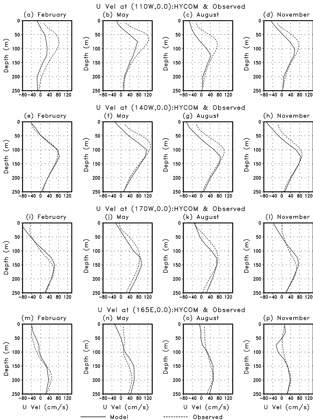
Fig. 6. The model and observed ADCP zonal velocity ( \text{cm s}^{-1} ) during boreal winter (February), spring (May), summer (August) and fall (November) respectively at the locations (110°W, 0) (a–d), (140°W, 0) (e–h), (170°W, 0) (i–l), and at (165°E, 0) (m–p) in the upper 250m for the model (solid lines) and observations (dashed lines).
