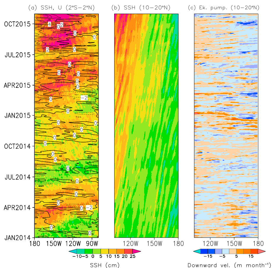
Figure 3. (a) Anomalies of SSH (shaded) and zonal 10 m wind (contours) averaged between 2^{\circ}\text{S} and 2^{\circ}\text{N} . (b) Same as Figure 3a except wind anomalies are not shown and SSH is averaged in the 10^{\circ}\text{N} – 20^{\circ}\text{N} band centered on Patricia (shown in Figure 1). (c) Same as Figure 3b except Ekman pumping velocity (positive downward). The x axis (longitude) in Figures 3b and 3c for has been reversed to show the westward propagating Rossby wave signal resulting from reflection at the eastern boundary.
