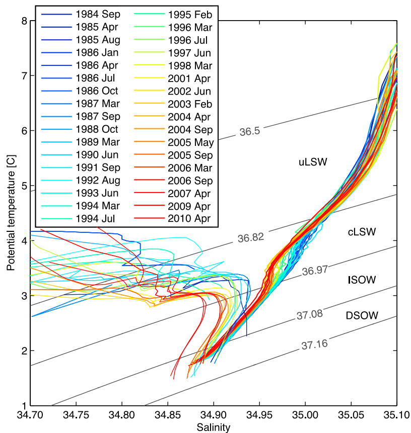
Figure 5. Temperature-salinity diagram of the water mass properties at the Abaco line (thick lines), with one line for each hydrographic section based on averaging water properties along \sigma_2 surfaces within 100 km of the continental shelf. The thin lines depict the water mass properties in the Labrador Sea, with a 9 year lead. The black lines are the \sigma_2 isopycnals that delineate the four different water masses. The freshening of the cLSW at Abaco in 1994–1996 is visible, as well as the increase in salinity of the upper Labrador Sea Water (uLSW) at that time. The same freshening of cLSW can be seen in the Labrador Sea, with a much larger spread in salinity.
