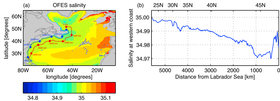
Figure 11. (a) Map of cLSW salinity in the OFES model, computed by depth-averaging the salinity between the \sigma_2 = 36.82 \text{ kg/m}^3 and \sigma_2 = 36.97 \text{ kg/m}^3 isopycnal surfaces, on the same color scale as the map of cLSW salinity in the climatologies (Figure 8). The range of salinity is much smaller in OFES than in the climatologies, but the shape of the MOW tongue and the Labrador Sea minimum is similar. (b) The salinity along the western continental shelf (blue line in Figure 11a) increases approximately linearly from 45^\circ\text{N} to 25^\circ\text{N} in the OFES model, also similar to what was found in the two climatologies (Figure 8). One difference between the climatologies and OFES, however, is a local maximum in salinity between the Grand Banks and the northern Labrador Sea. This maximum is also responsible for the local minimum in salinity at the 300 km point in Figure 11b.
