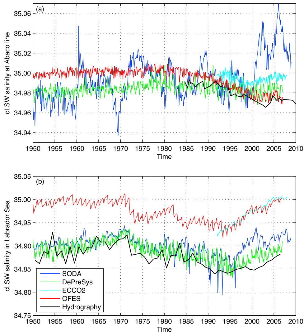
Figure 10. Comparison of salinity of the four different numerical models with the hydrography for (a) the Abaco line and (b) the Labrador Sea, computed by depth-averaging the salinity between the \sigma_2 = 36.82 \text{ kg/m}^3 and \sigma_2 = 36.97 \text{ kg/m}^3 isopycnal surfaces. At the Abaco line, OFES follows the hydrography best, with the variability in SODA too large and the decrease in salinity after the 1990s not captured by DePreSys and ECCO2. In the Labrador Sea, SODA and DePreSys follow the hydrography much better. ECCO2 and OFES have a similar decadal variability, but suffer from a bias.
