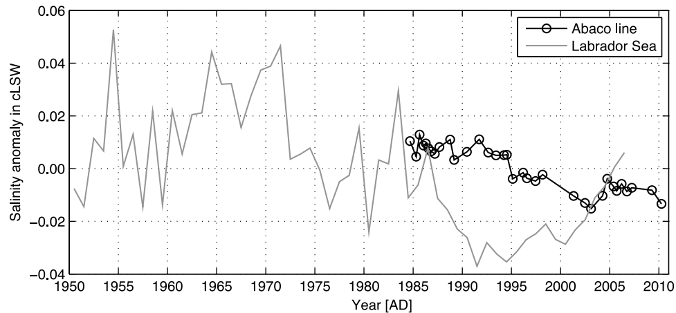
Figure 6. The evolution of salinity anomalies in the cLSW density class (between the \sigma_2 = 36.82 \text{ kg/m}^3 and \sigma_2 = 36.97 \text{ kg/m}^3 isopycnals) at the Abaco line and in the Labrador Sea. The latter data set was compiled by Van Aken et al. [2011]. The decrease in salinity in the Labrador Sea between 1984 and 1995 leads to a decrease in salinity at the Abaco line starting in 1995. Although not statistically significant, there is a 0.80 correlation at a 9 year lag between the Labrador Sea and the Abaco line, with the amplitude of decadal variability decreased by a factor 2.
