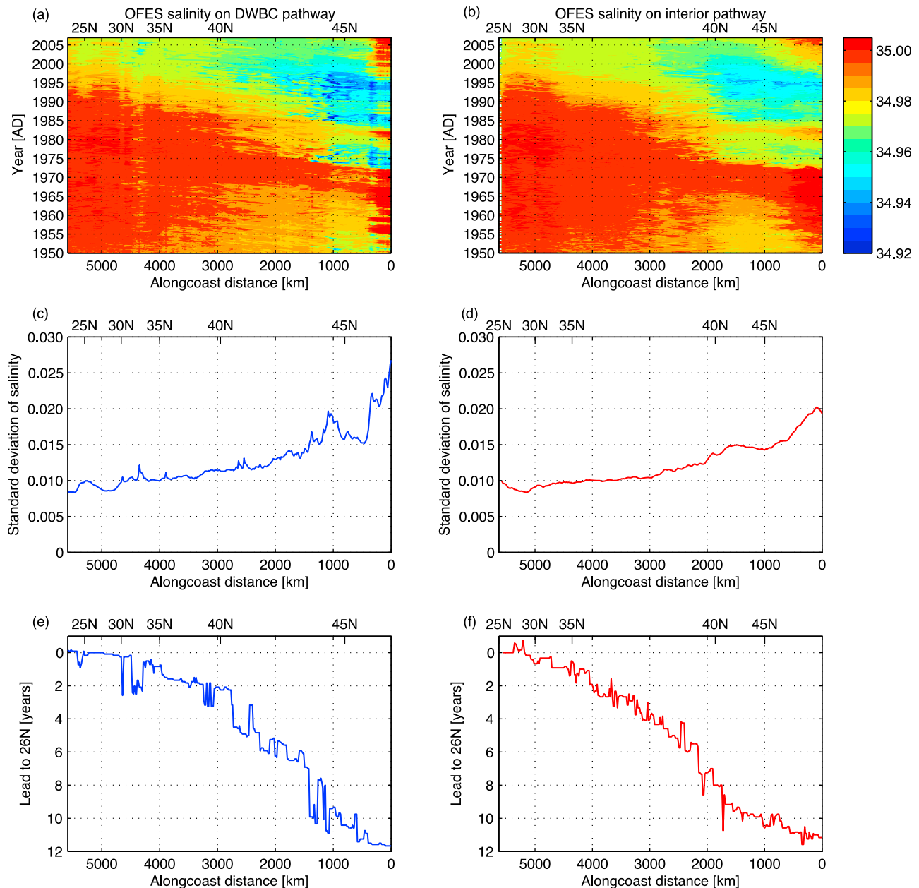
Figure 12. The advection of salinity anomalies along (left) the DWBC and in (right) the interior pathway, defined as the blue and red lines in Figure 11b. (a and b) Hovmöller diagram of salinity from the Labrador Sea (Figure 12, right) to the Abaco line (Figure, 12 left) in the OFES model. (c and d) The standard deviation in salinity at each grid point for the two pathways. Most of the variability in salinity is damped before the signal reaches 40°N. The decrease in variability is a factor 2 to 3. (e and f) The lead, in years, at which the time series of salinity at each point along the continental shelf has the largest correlation with the time series of salinity at 26°N. The lead increases moving northeastward.
