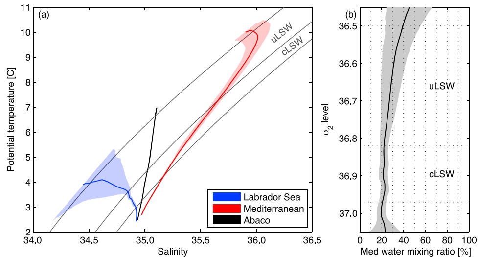
Figure 9. The mixing fractions of Labrador Sea Water and Mediterranean Outflow Water at the Abaco line from the HydroBase2 climatology. (a) Temperature-salinity diagrams for the HydroBase2 profiles in the Labrador Sea (blue), the Gulf of Cádiz (red), and at the Abaco line (black). See Figure 1 for the locations where these profiles are computed. The colored lines denote mean profiles; the shaded areas denote standard deviations around the means (calculated on \sigma_2 levels). There is no shading for Abaco since the region is one single grid point. The gray lines are the \sigma_2 isopycnals that delineate the different water masses. (b) The percentage of Mediterranean Water needed to explain the Abaco profile as a function of \sigma_2 , under the assumption that the rest of the water is Labrador Sea Water. The gray area is the 1 \sigma confidence interval. For cLSW, the fraction of Mediterranean Water at Abaco is slightly more than 20%.
