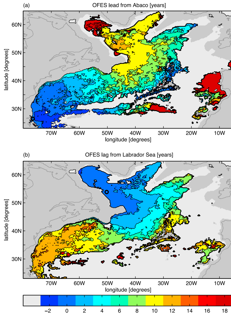
Figure 14. Advection timescales in the OFES model to (a) the Abaco line and from (b) the Labrador Sea, determined from the lag at which correlation is highest between the time series of salinity at the base point (the black circles) and the time series of salinity at any other point in the North Atlantic in the cLSW density range. Areas where the correlation is lower than 0.75 are shaded light gray and areas where no correlations have been computed are shaded dark gray. In the model, the lag between the Labrador Sea and the Abaco line is 10–12 years.
