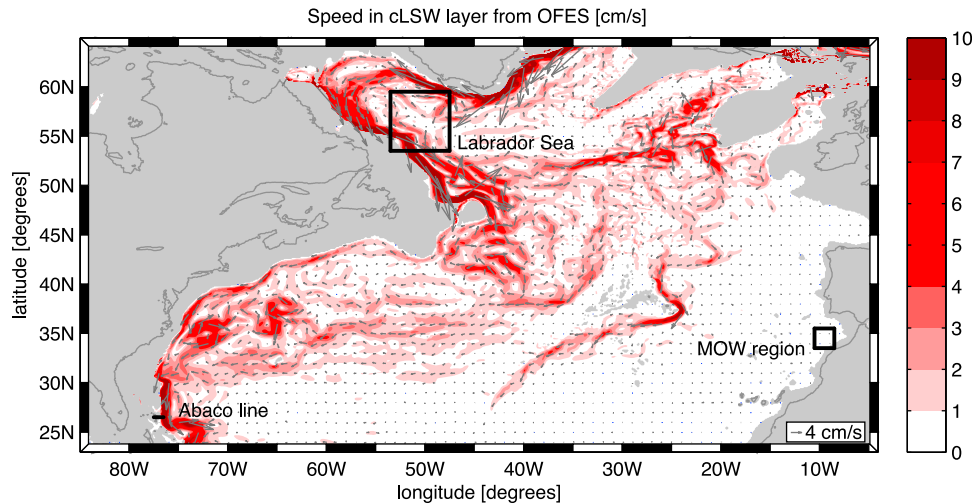
Figure 1. Classical Labrador Sea Water (cLSW) map of the North Atlantic Ocean depicting the regions of interest for this study (the Abaco line, the Labrador Sea, and the Mediterranean Outflow Water region) on top of the climatological velocity field in the OFES model climatology, depth-averaged between the \sigma_2 = 36.82 \text{ kg/m}^3 and \sigma_2 = 36.97 \text{ kg/m}^3 isopycnal surfaces. Velocities in this layer are typically 4 cm/s in the Deep Western Boundary Current. At 5000 km, this implies a lag between the Labrador Sea and Abaco line of approximately 4 years. Molinari et al. [1998], however, found a lag of 10 years; a timescale which is confirmed in this study.
