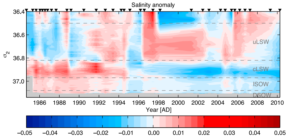
Figure 4. Hovmoller plot of the salinity anomaly obtained by averaging the salinity in the first 100 km offshore along \sigma_2 isopycnals in the DWBC at the Abaco line, with the water mass classification in dashed lines. The black triangles at the top indicate when the sections were occupied. It appears that on decadal timescales cLSW and the two types of overflow water become fresher, while uLSW becomes saltier.
