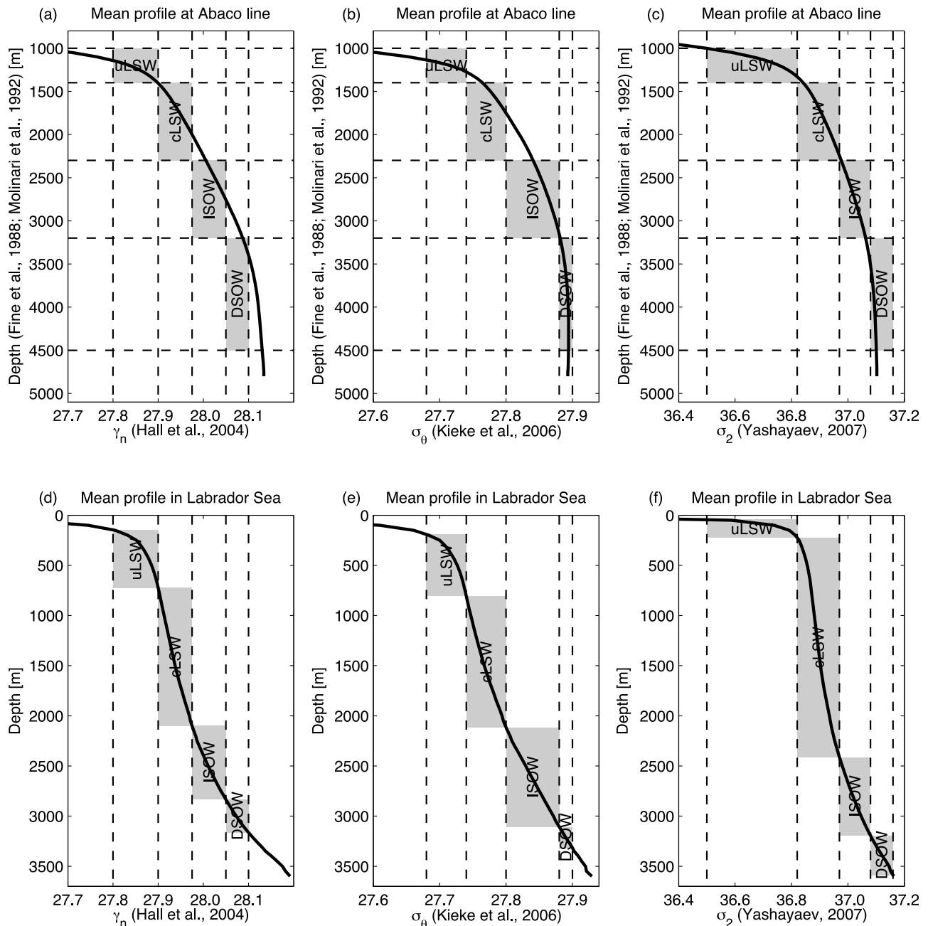
Figure 3. The mean profile of neutral density ( \gamma_n ), \sigma_\theta , and \sigma_2 (a–c) in the Deep Western Boundary Current (DWBC) off Abaco and (d–f) the Labrador Sea. Fine and Molinari [1988] and Molinari et al. [1998] proposed a division in water mass classes based on the hydrography at the Abaco line itself using depth levels (vertical axes in Figures 3a–3c). In the Labrador Sea, each of the different density coordinates has a different classification (horizontal axes), proposed by different authors. Part of the differences between the depths of the water masses at the Abaco line can be related to differences in the depths of the water masses in the Labrador Sea itself (Figures 3d–3f). The classification that best relates the water masses in the Labrador Sea with those at Abaco is that based on \sigma_2 isopycnals (Figures 3c and 3f).
