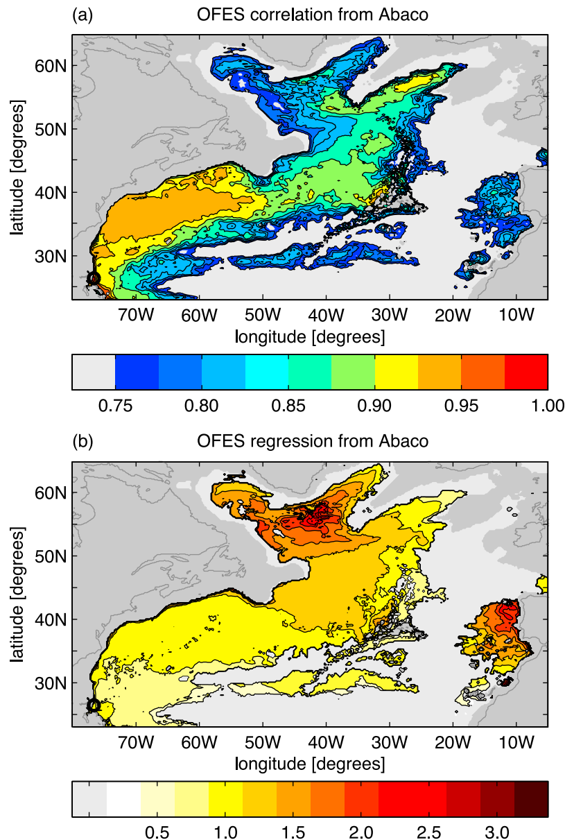
Figure 13. Maps of (a) lagged correlation and (b) regression in the OFES model between the time series of salinity at the Abaco base point (the black circles) and the time series salinity at any other point in the North Atlantic in the cLSW density range. Areas where the correlation is lower than 0.75 are shaded light gray and areas where no correlations have been computed are shaded dark gray. In the model, the correlation between the Labrador Sea and the Abaco line is around 0.8, and the regression is approximately 2. This agrees with the results from the hydrographic time series (Figure 6).
