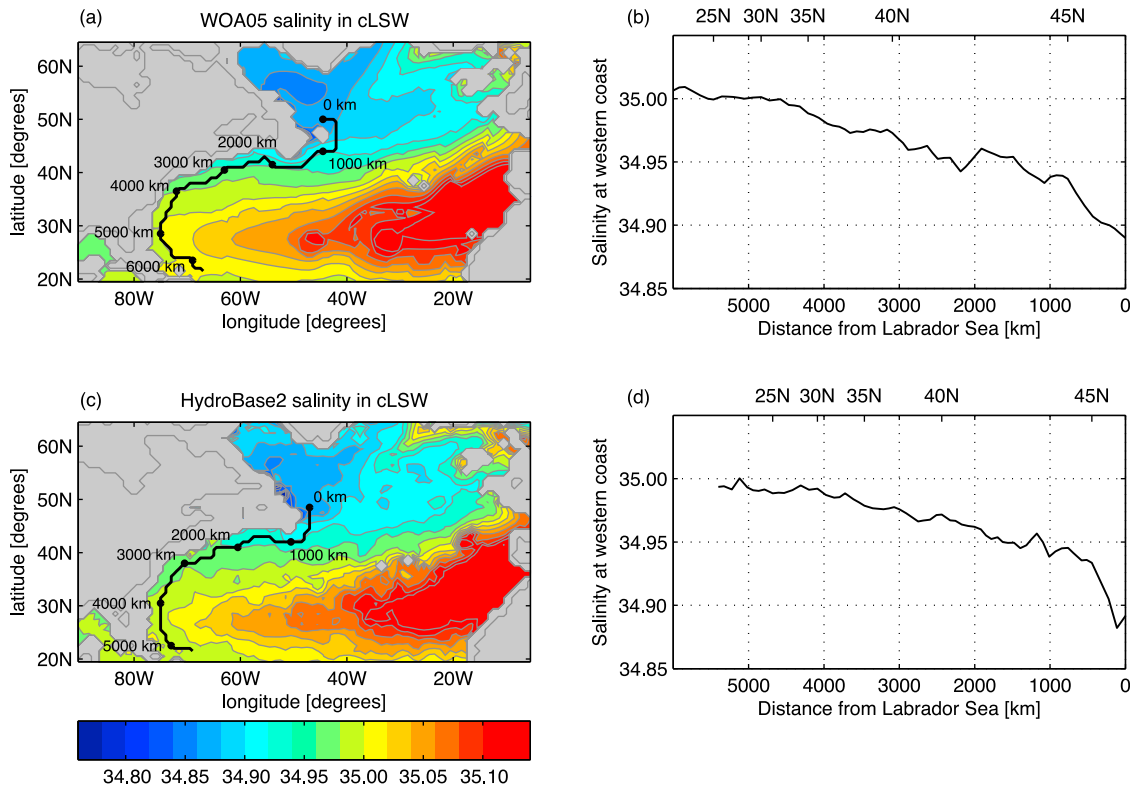
Figure 8. Map of cLSW salinity, computed by depth-averaging the salinity between the \sigma_2 = 36.82 \text{ kg/m}^3 and \sigma_2 = 36.97 \text{ kg/m}^3 isopycnal surfaces in (a) the World Ocean Atlas 2005 and (c) the HydroBase2 climatology. The amount of small-scale variability is different between the two climatologies, but the large-scale patterns are similar. Note that the color scale is cut off at 35.14, the core of the MOW is saltier than that at 35.30. The salinity along the western Atlantic continental shelf ((b) and (d)), calculated along the black lines in Figures 8a and 8c) shows that for both climatologies the salinity increases approximately linear between 45^\circ\text{N} and 25^\circ\text{N} .
