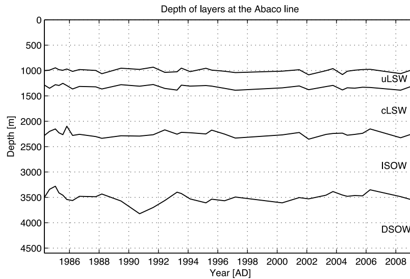
Figure 7. Evolution of layer thickness for the four different water masses at the Abaco line. Unlike in the Labrador Sea, where the thickness of uLSW and cLSW vary by more than 1000 m on decadal timescales [Kieke et al. , 2006], there is little variability in the thickness of the Labrador Sea water masses at the Abaco line.
