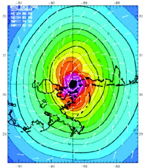
Observed Max. Surface Wind: 129 kts, 8 nm NE of center based on 0430 z 1 sfc measurement Analyzed Max. Wind: 127 kts, 7 nm NE of center Experimental research product of NOAA / AOML / Hurricane Research Division
