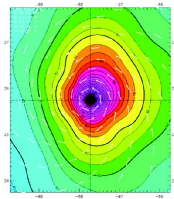
Observed Max. Surface Wind: 139 kts, 14 nm NE of center based on 1422 z AFREC sfc measurement Analyzed Max. Wind: 139 kts, 14 nm NE of center Experimental research product of NOAA / AOML / Hurricane Research Division
