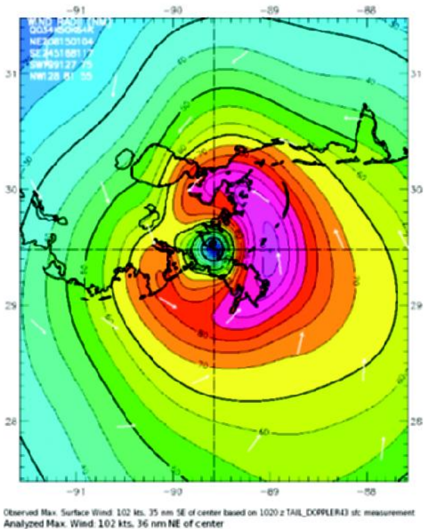
c) Hurricane Katrina 1200 UTC 29 AUG 2005 Max 1-min sustained surface winds (kt) Valid for marine exposure over water, open terrain exposure over land Analysis based on: SPOSNDX_01 150 from 085 - 135 Z; FCNP_TOWER from 042 - 155 Z; VAD_180 from 055 - 155 Z; QSCAT from 138 - 152 Z; DWP from 155 - 132 Z; AOC from 056 - 155 Z; SFIR43 from 056 - 135 Z; MOORED_BUOY from 055 - 140 Z; METAR from 050 - 135 Z; CTRM from 056 - 140 Z; DCS_SIVR from 152 - 152 Z; TAIL_DOPPLER43 from 152 - 134 Z; RADIC from 055 - 155 Z; DUAL_DOPPLER from 152 - 152 Z; WINDHAT from 057 - 140 Z; 1200 z position interpolated from 1132 Army Corps; mslp = 923.0 mb
