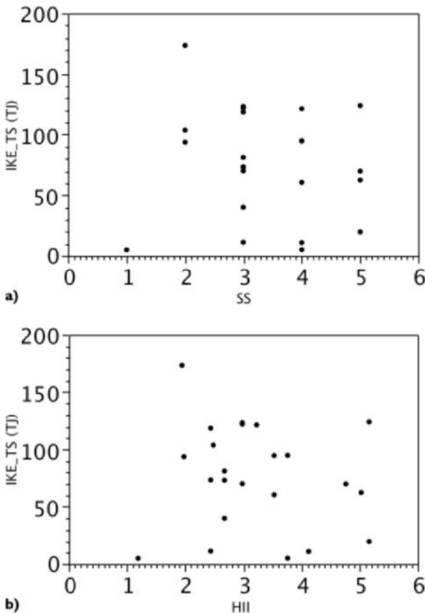
FIG. 6. Comparison of IKE_{TS} to (a) SS and (b) HII based on best track V_{ms} .
