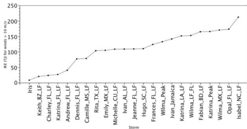
Fig. 2. Storm-scale integrated kinetic energy for winds > 10 m s -1 . Letters refer to state or country abbreviations and landfall (LF) status or peak H*Wind intensity follow each storm name.
