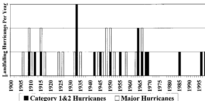
Fig. 7. Number of hurricanes that made landfall in Cuba, 1900–1998
