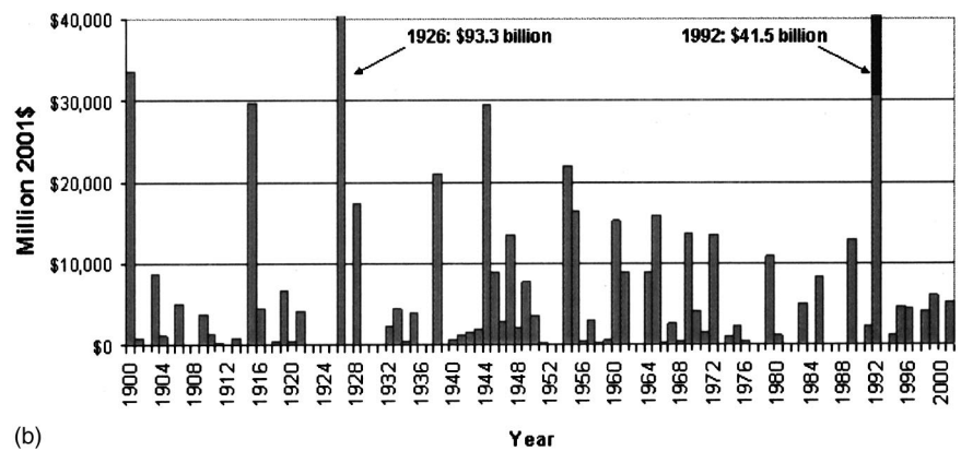
Fig. 3. 1900–2001 U.S. hurricane damage: (a) adjusted for inflation; (b) normalized to 2001 values
