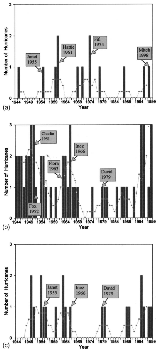
Fig. 2. 1944–1999 time series of (a) Central American, (b) Northern Caribbean, and (c) Southern Caribbean hurricanes (line represents moving 5-year average)
