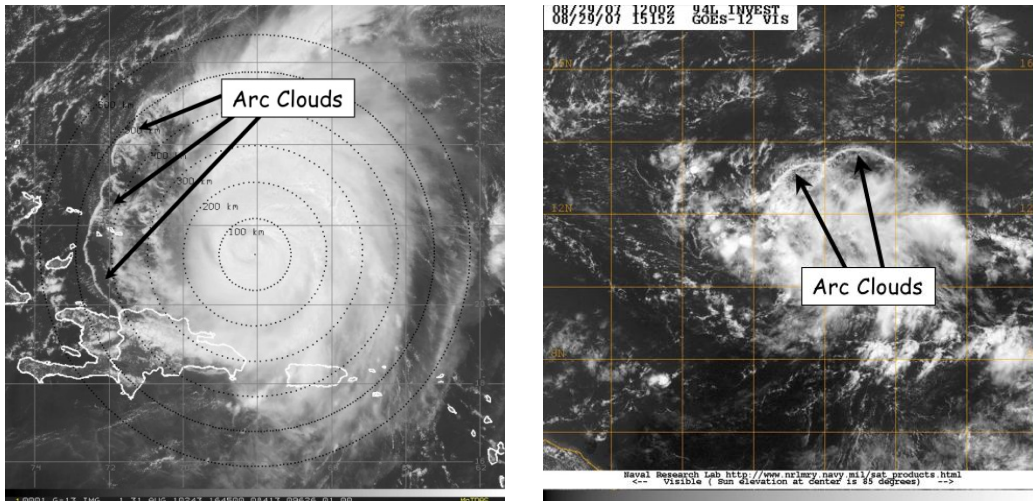
Figure 21-1: GOES visible satellite imagery showing arc clouds racing away from the convective cores of (left) 2003 Hurricane Isabel and (right) 2007 Pre-Tropical Depression Felix.
