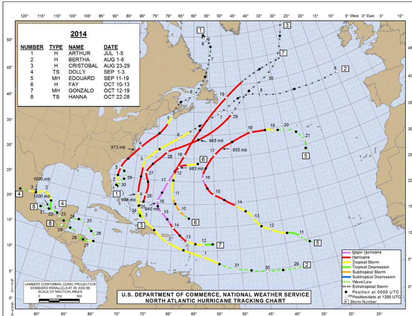
Figure 1: Tracks of the (sub)tropical storms and hurricanes of the 2014 Atlantic Hurricane Season.
