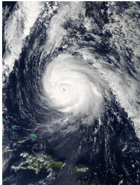
NASA MODIS VISIBLE IMAGE OF HURRICANE GONZALO AT 1745 UTC 16 OCTOBER 2014
