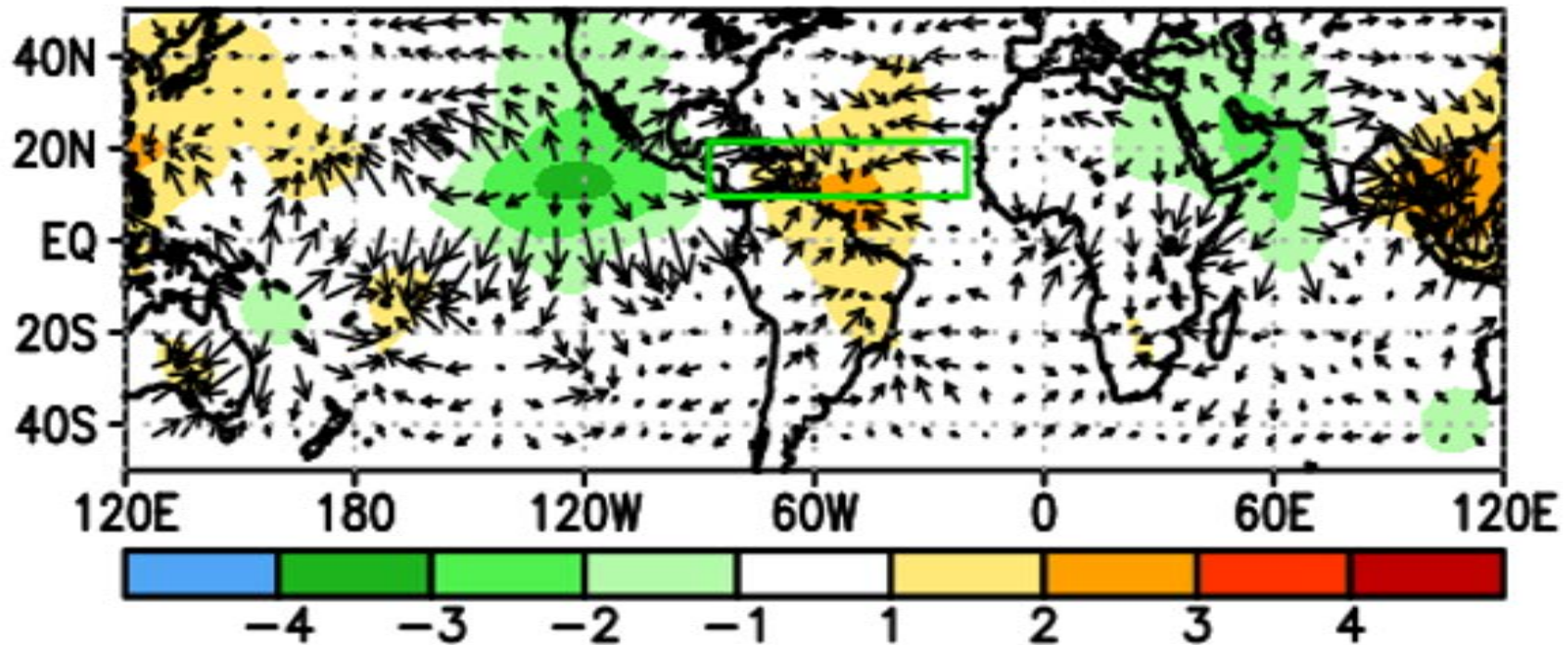
Figure 3: 200 mb anomalous velocity potential ( 10^6 \text{ m}^2 \text{ s}^{-1} ) and divergent wind for August through October of 2014. The green box indicates the Main Development Region. Anomalies are based on the 1981-2010 climatology. Figure courtesy of Gerry Bell (Climate Prediction Center).
