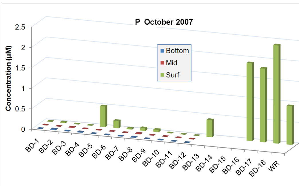
Figure 31: October 2007 orthophosphate concentrations for the Boynton-Delray water quality monitoring stations.
