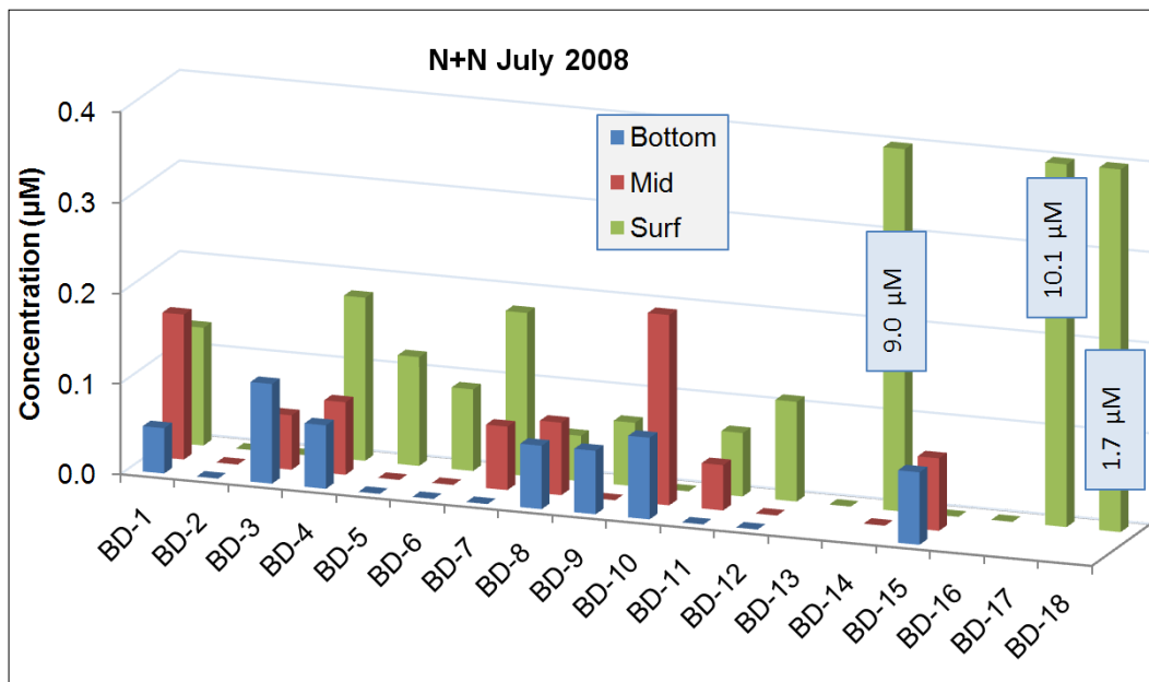
Figure 104: July 2008 nitrate+nitrite concentrations for the Boynton-Delray water quality monitoring stations. Concentrations higher than 0.4 µM are specifically denoted.
