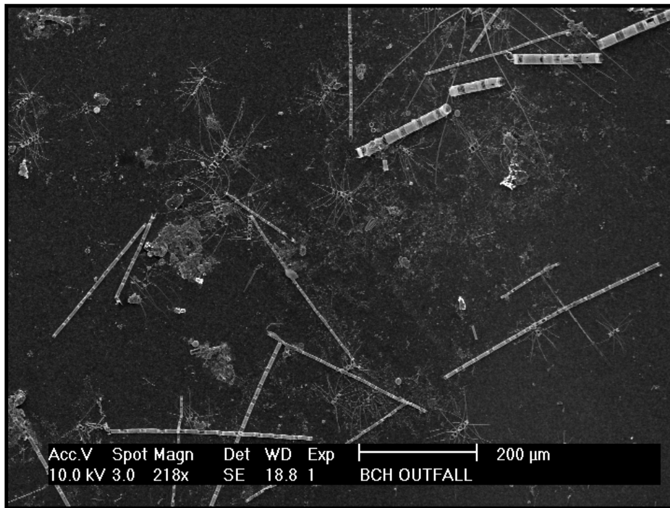
Figure 5: Centric diatom distribution in the >5 μm size fraction from Boynton Inlet station BD-13A.
