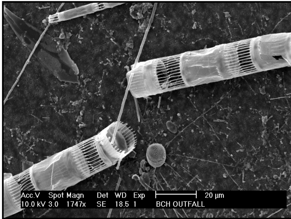
Figure 4: Detail of Skelatonema sps. in the >5 μm size fraction from Boynton Inlet station BD-13A.
