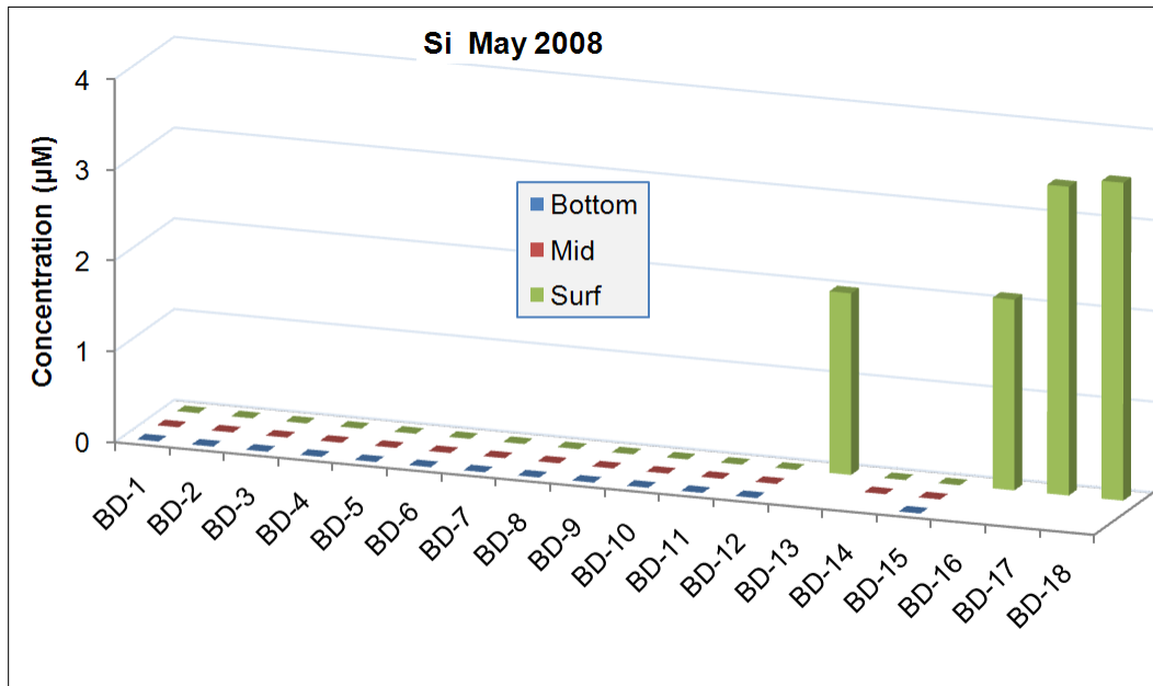
Figure 78: May 2008 silicate concentrations for the Boynton-Delray water quality monitoring stations.
