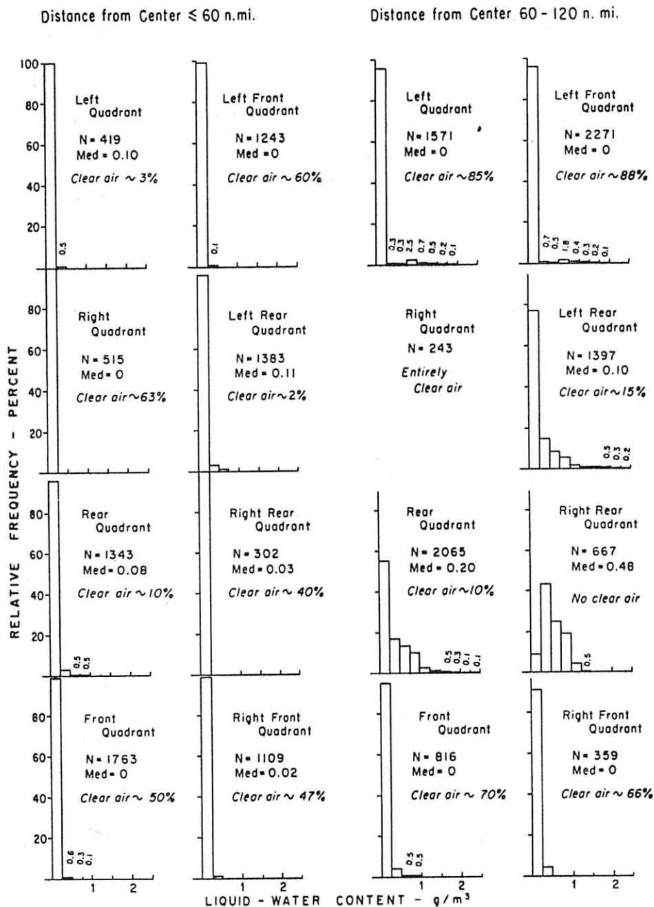
Figure 9. - Frequency distributions of water content (1-sec. means) in tropical storm Becky, by quadrant. Division into sectors according to figure 2.
