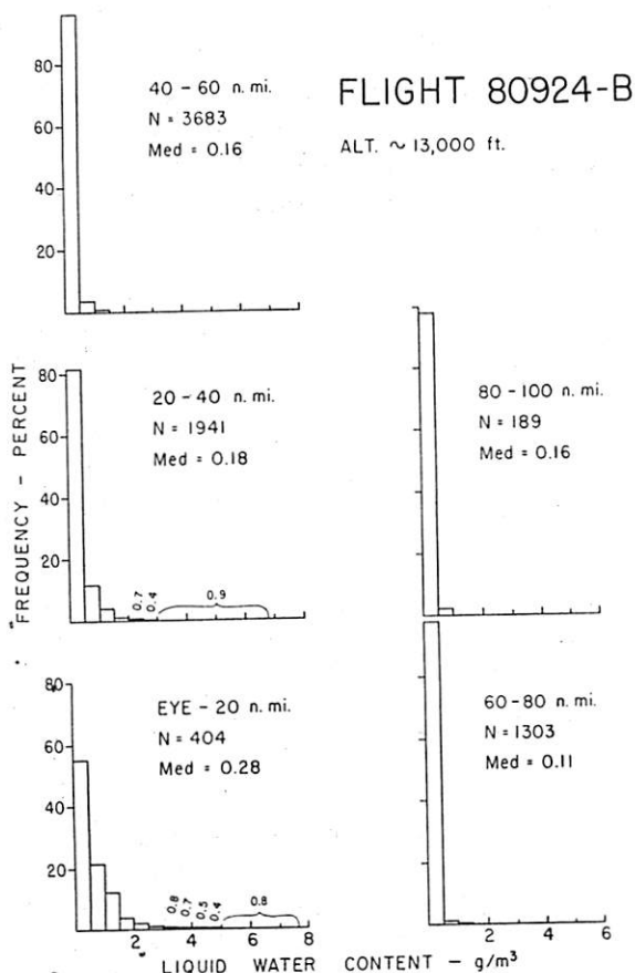
Figure 24. - Frequency distributions of water content (1-sec. means) for 20-mi. wide annular rings at 13,000 ft. in hurricane Helene on September 24.
