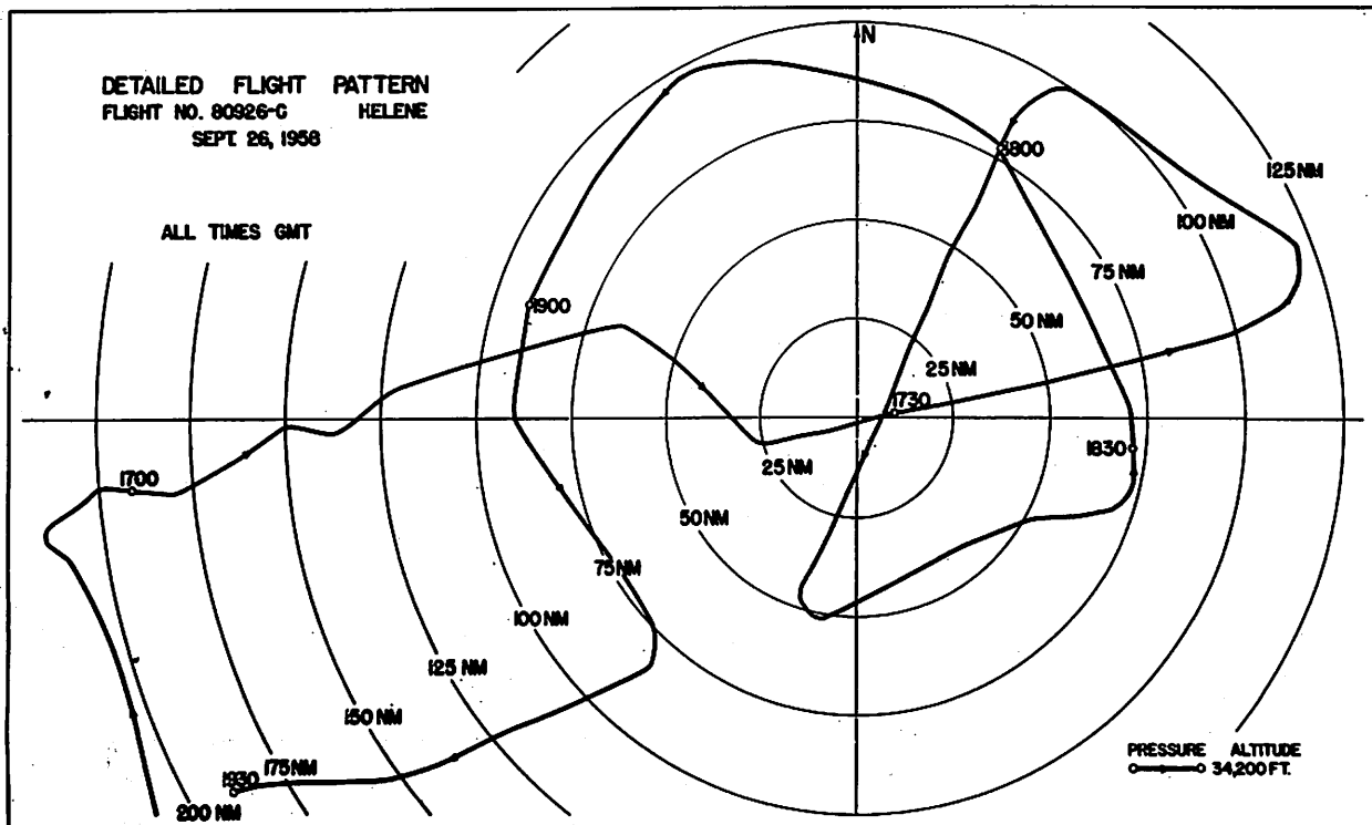
Figure 3. - Flight paths of NHRP aircraft on September 26: (a) at 800 mb., (b) at 237 mb.
