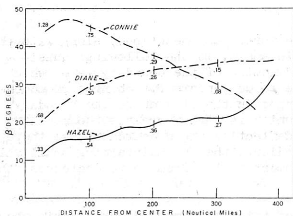
Figure 6. - Cross-isobar angle (degrees) for three hurricanes with pressure gradient per unit mass shown in units of \text{cm. sec.}^{-2} .
