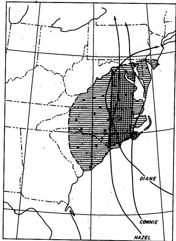
Figure 1. - Track of three hurricanes and area of analysis.
