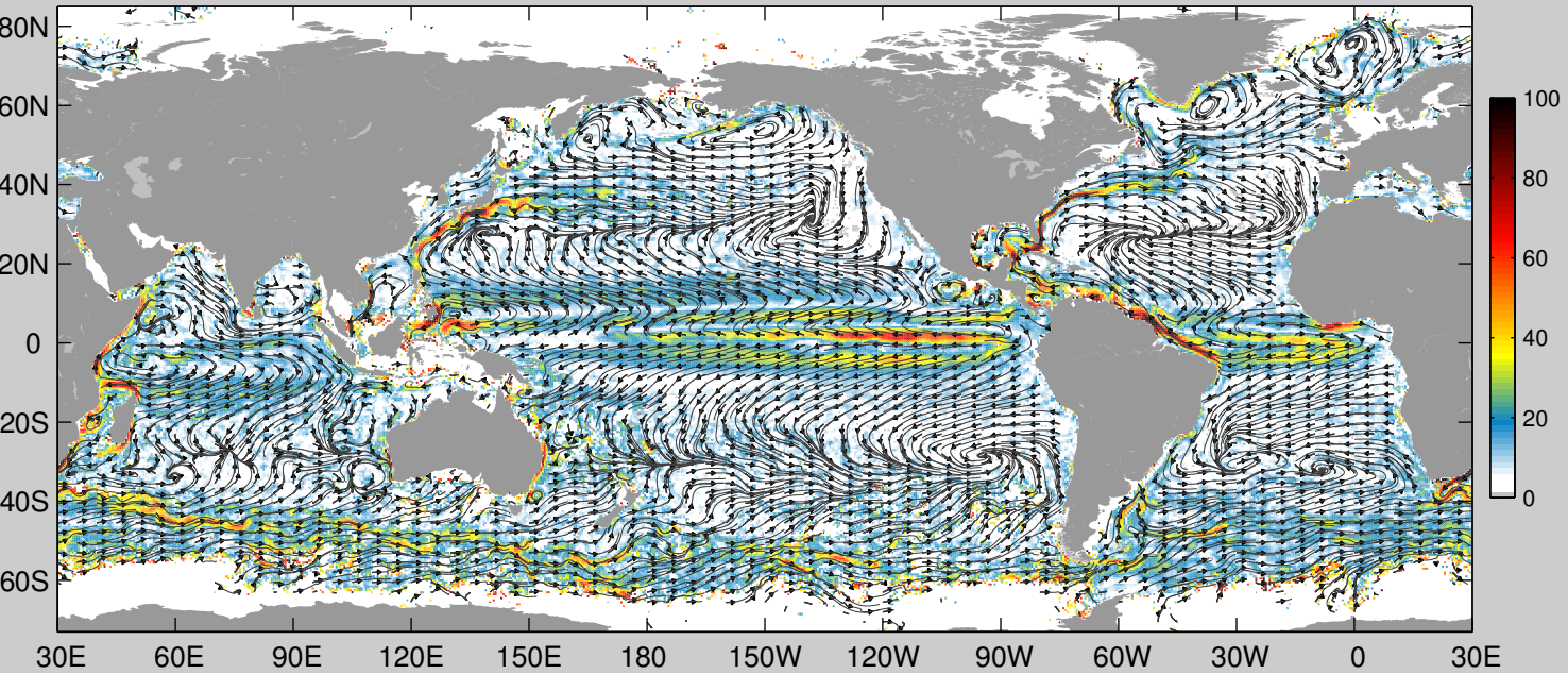
Annual mean drifter speed (cm/s)
