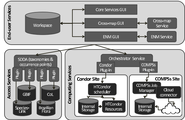
Fig. 2. Use Case Architecture Deployment
