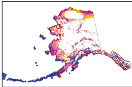
Figure 4. Estimated annual average wind power at 50 meters elevation. Areas with resource potential classified as outstanding or superb are almost exclusively offshore. Map by National Renewable Energy Laboratory [6].
