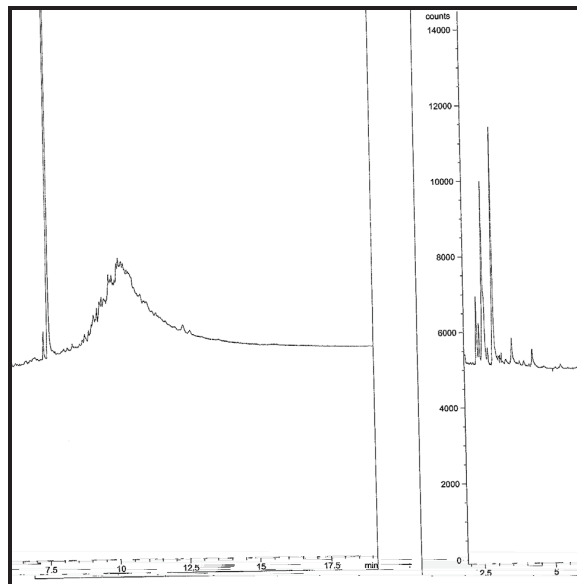
Chromatogram for sediment core BP-24 (359-360 cm).
