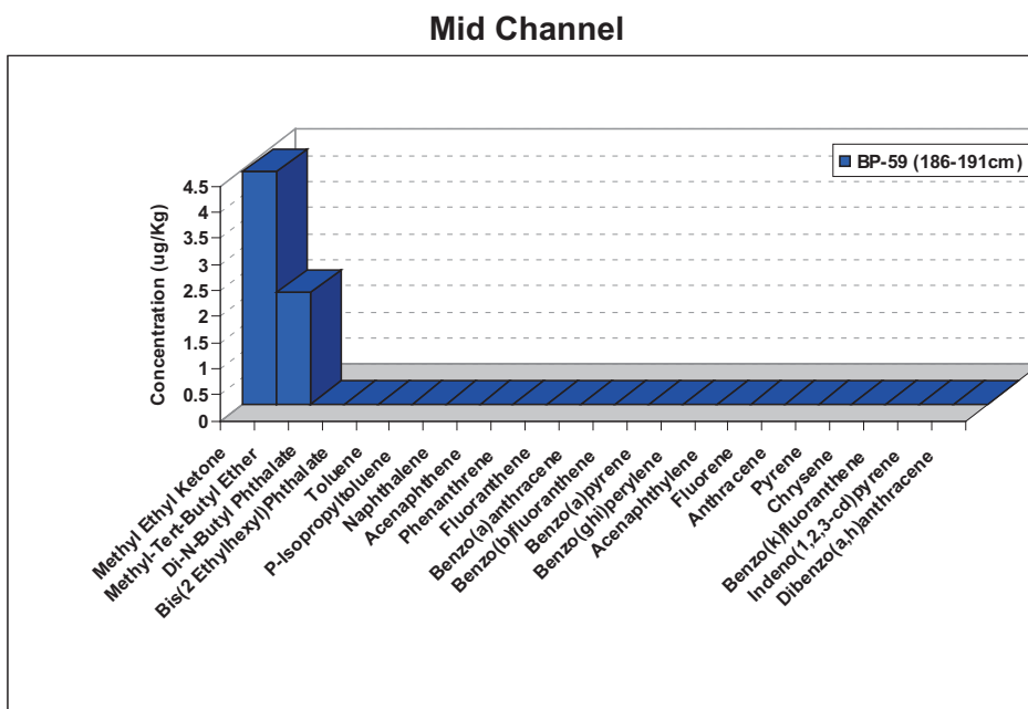
Figure 15A: Blind Pass Mid Channel speciation data indicating concentrations of ether and ketone in BP-59 (186-191 cm).
