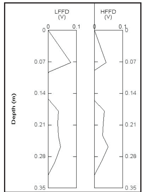
Figure 98: FFD probe analysis of BP-84.
