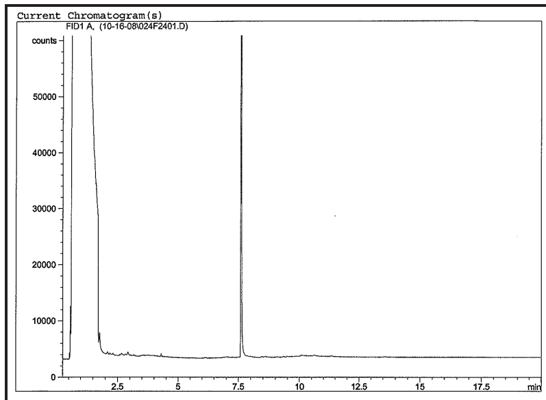
Chromatogram of sediment core JP-11-2 (148-153 cm).
