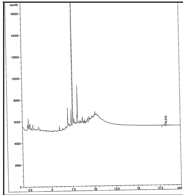
Chromatogram for sediment core BP-31 (265-271 cm).
