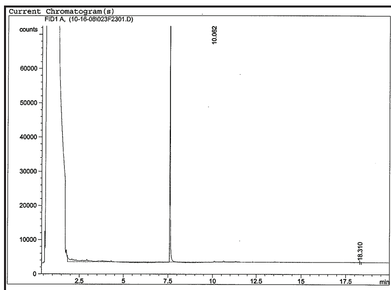
Chromatogram of sediment core JP-13 (65-70 cm).
