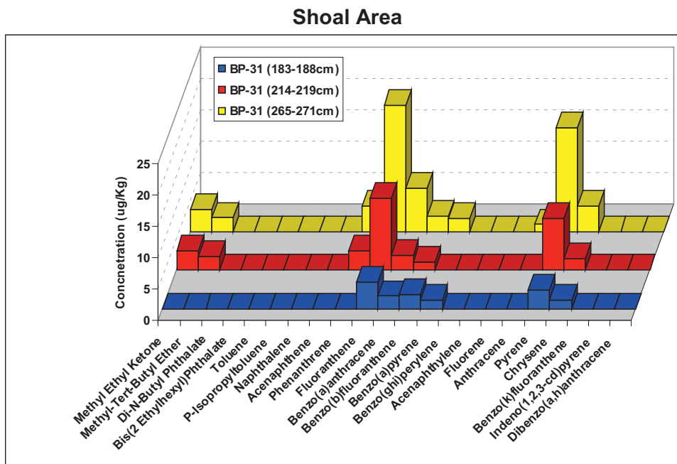
Figure 17C: Individual petroleum hydrocarbon speciation of BP-31 (183-188 cm, 214-219 cm, and 265-271 cm) from the Shoal area of Blind Pass.
