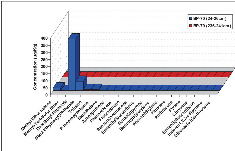
Figure 15B: Evidence of phthalates and low concentrations of ketones and toluene in BP-70
