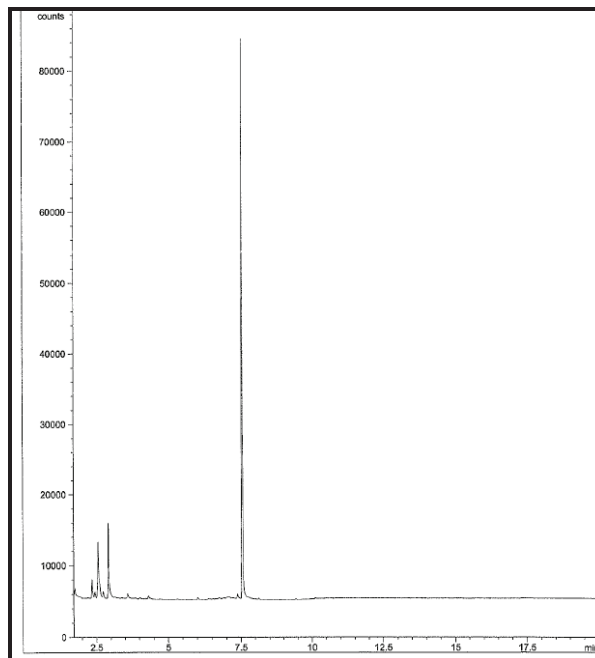
Chromatogram for sediment core BP-91 (238-243 cm).
