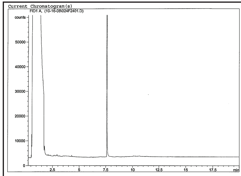
Chromatograph of sediment core JP-12-2 (120-125 cm).
