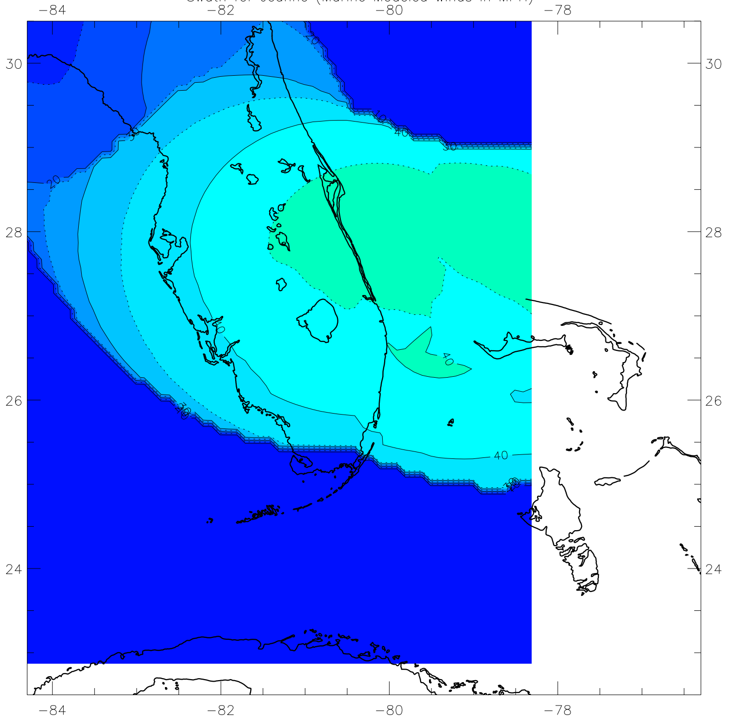
Swath for Jeanne (Marine Modeled winds in MPH)
