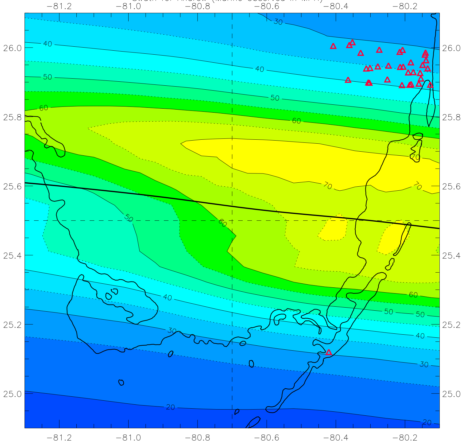
Swath for Andrew (Marine Observed in MPH)
