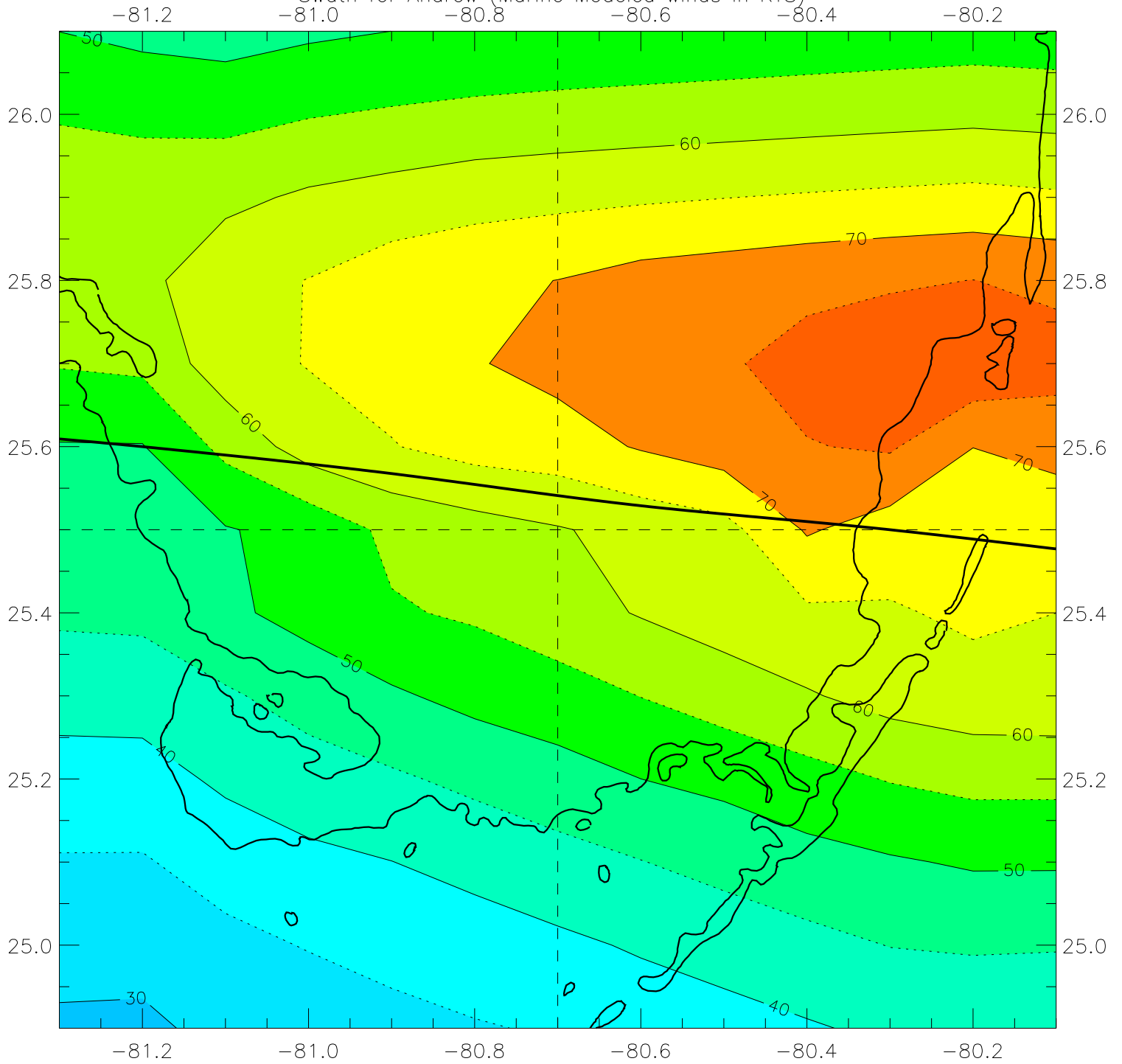
Swath for Andrew (Marine Modeled winds in KTS)
