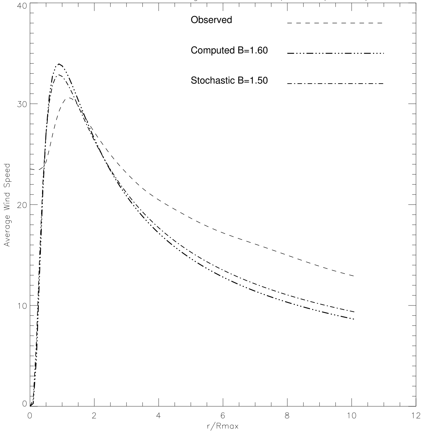
Katrina 2100Z— Average Wind versus r/R_{max} (surface)
