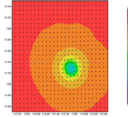
Hurricane Patricia 20151022 1830Z Mean Sea-level Pressure [hPa]
