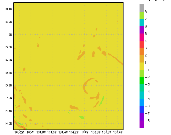
Hurricane Patricia 20151022 1730Z 925 hPa Vertical Velocity [m/s]
