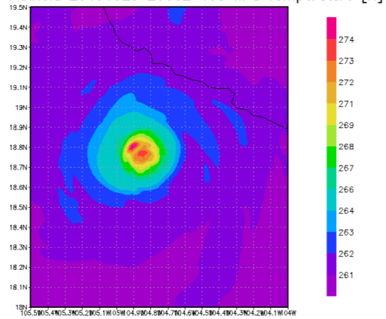
Hurricane Patricia 20151023 2000Z 400 hPa Temperature [K]
