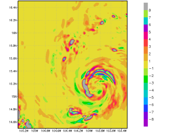
Hurricane Patricia 20151022 1730Z 300 hPa Vertical Velocity [m/s]
