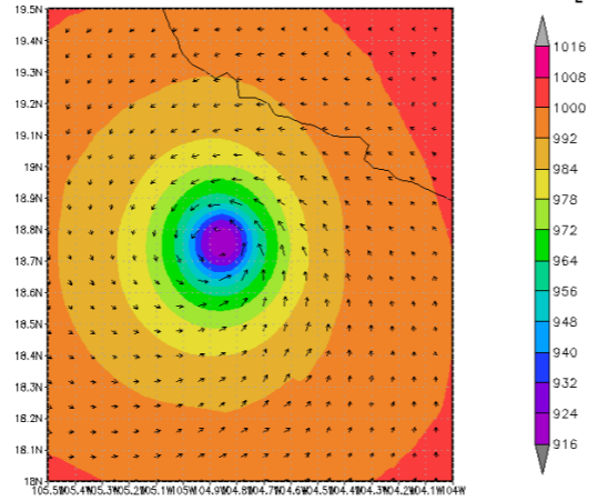
Hurricane Patricia 20151023 2000Z Mean Sea-level Pressure [hPa]
