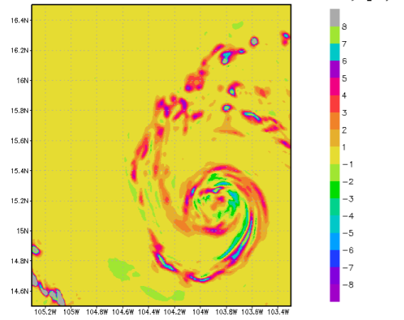
Hurricane Patricia 20151022 1730Z 700 hPa Vertical Velocity [m/s]
