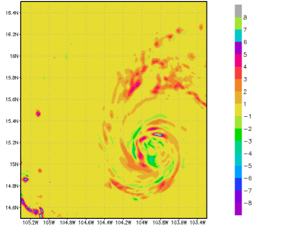
Hurricane Patricia 20151022 1730Z 850 hPa Vertical Velocity [m/s]
