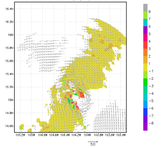
15102211 PATRICIA at 0.5 km (m/s) Valid 20151022 1739Z
