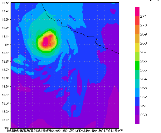
Hurricane Patricia 20151023 2100Z 400 hPa Temperature [K]
