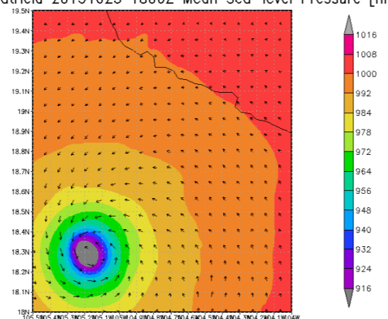
Hurricane Patricia 20151023 1800Z Mean Sea-level Pressure [hPa]
