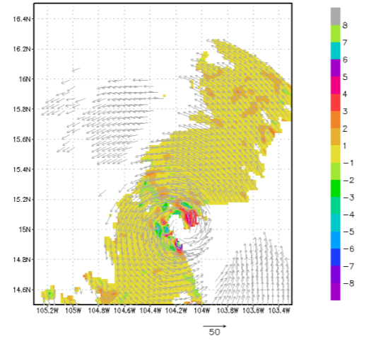
15102211 PATRICIA at 1.5 km (m/s) Valid 20151022 1739Z
