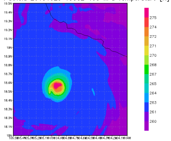
Hurricane Patricia 20151023 1930Z 400 hPa Temperature [K]
