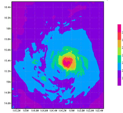
Hurricane Patricia 20151022 1900Z 400 hPa Temperature [K]
