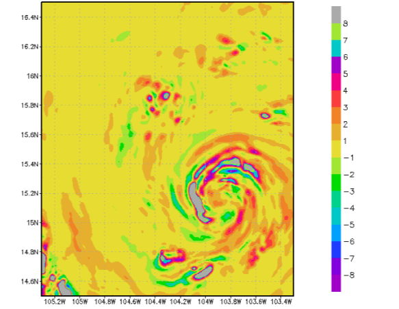
Hurricane Patricia 20151022 1730Z 250 hPa Vertical Velocity [m/s]
