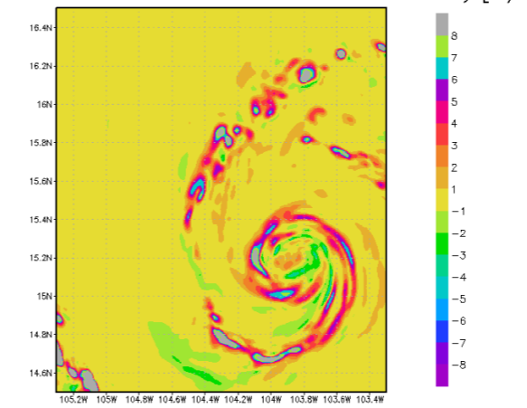
Hurricane Patricia 20151022 1730Z 400 hPa Vertical Velocity [m/s]
