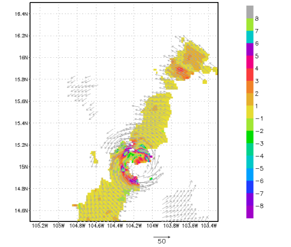
15102211 PATRICIA at 7 km (m/s) Valid 20151022 1739Z
