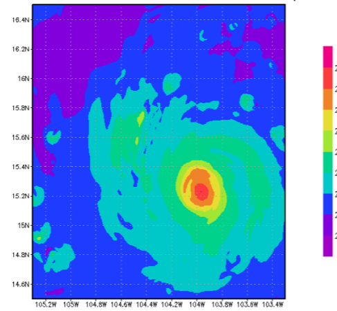
Hurricane Patricia 20151022 1800Z 400 hPa Temperature [K]
