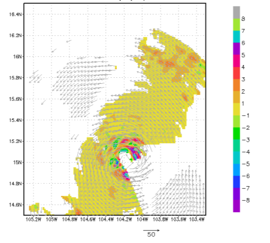
15102211 PATRICIA at 3 km (m/s) Valid 20151022 1739Z
