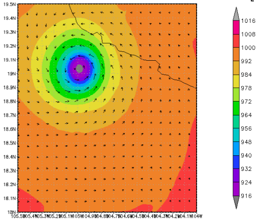
Hurricane Patricia 20151023 2100Z Mean Sea-level Pressure [hPa]
