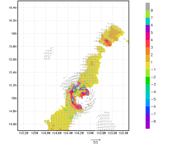
15102211 PATRICIA at 9 km (m/s) Valid 20151022 1739Z
