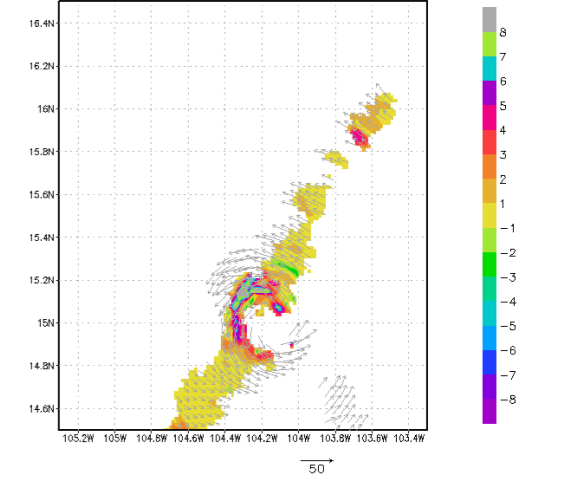
15102211 PATRICIA at 10 km (m/s) Valid 20151022 1739Z
