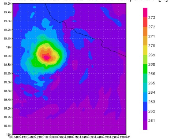
Hurricane Patricia 20151023 2030Z 400 hPa Temperature [K]
