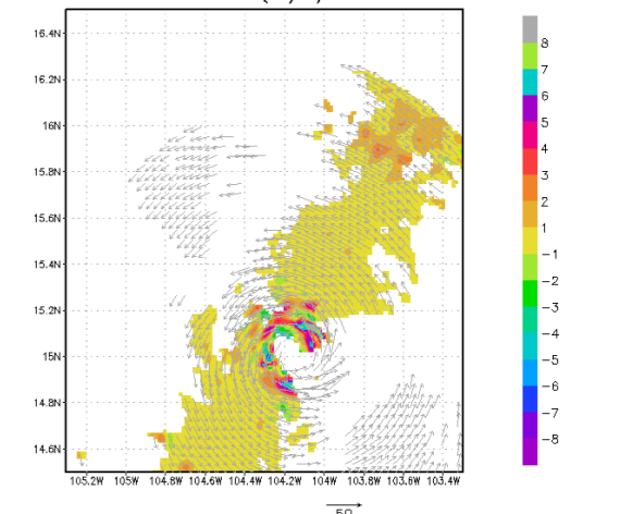
15102211 PATRICIA at 7 km (m/s) Valid 20151022 1739Z
