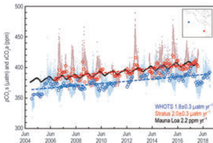
FIG. 3.27. Moored time-series observations of surface ocean seawater p\text{CO}_2 ( p\text{CO}_2\text{s} ) at the WHOTS (blue) and Stratus (red) sites in the subtropical Pacific (inset). Light colors are the high-resolution measurements and circles represent de-seasoned monthly means. Dashed lines represent trend of de-seasoned values. As a reference, the climate record of atmospheric \text{CO}_2 ( x\text{CO}_2\text{a} ) from Mauna Loa Observatory is shown in black (NOAA ESRL Global Monitoring Division, 2017).
