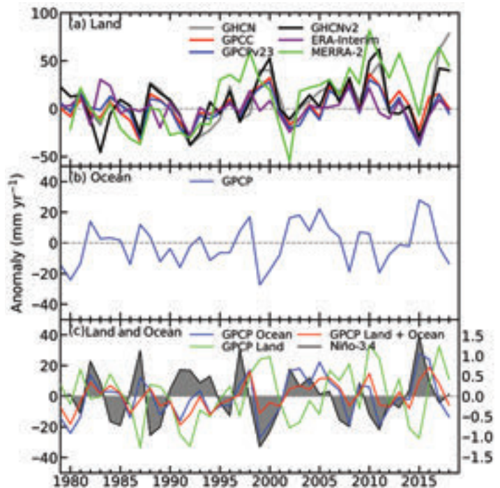
FIG. 2.20. Globally averaged precipitation anomalies ( \text{mm yr}^{-1} ) relative to the 1981–2010 base period over (a) land areas; (b) ocean areas; and (c) GPCP land, ocean, and combined time series overlaid with the Niño-3.4 index (right axis). Land time series for panel (a) were created using a proportional land/sea mask at the 1^\circ \times 1^\circ scale whereas ocean and land time series for panels (b) and (c) were created using a proportional land/sea mask at the 2.5^\circ \times 2.5^\circ scale.
